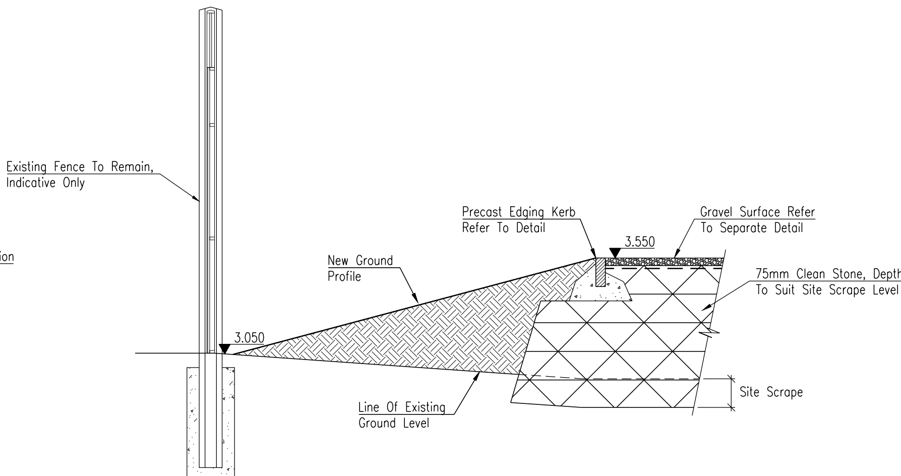
Section C-C Scale 1:20
