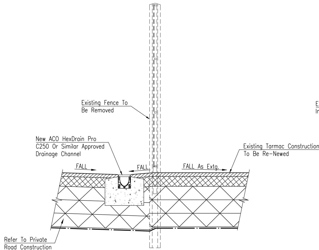
Section B-B - Local To Access Point Scale 1:20
