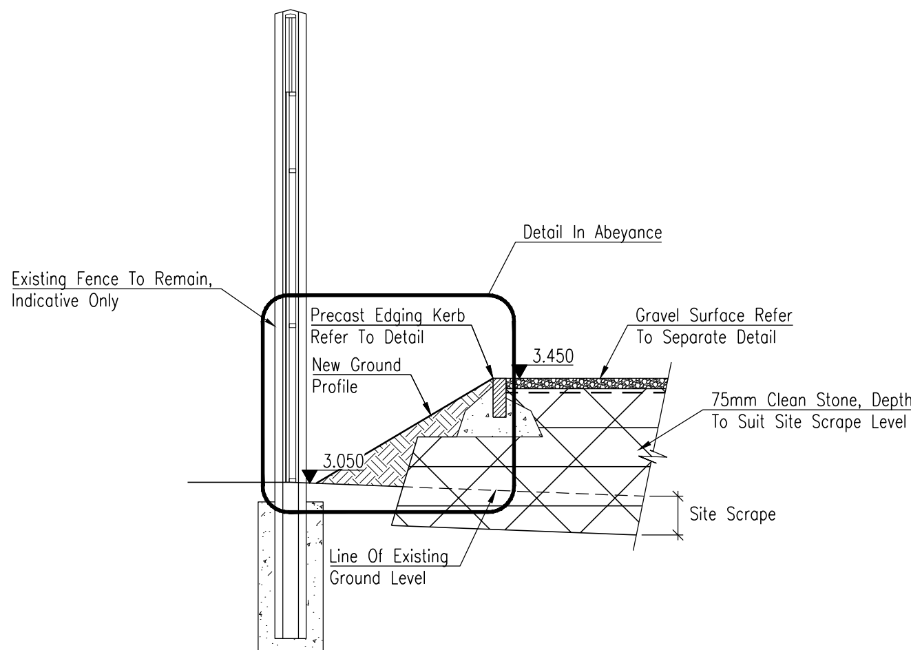
Section D-D Scale 1:20
