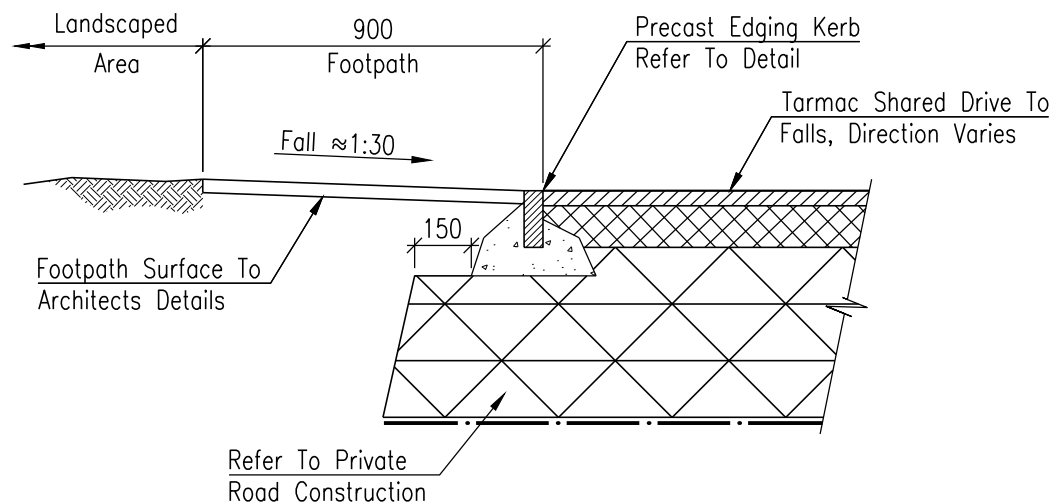
Typical Footpath Detail Scale 1:20
