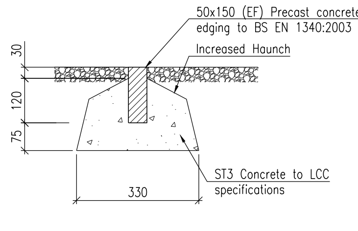
Edging Kerb Detail (50x150 EF) Within Gravel Areas Scale 1:10
