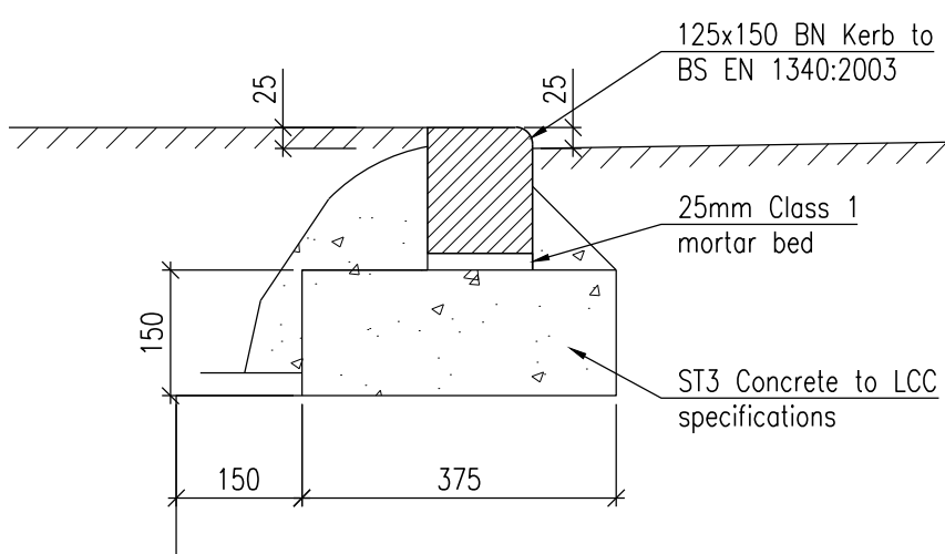
Typical Dropped Kerb Detail (125x150 BN) Scale 1:10
