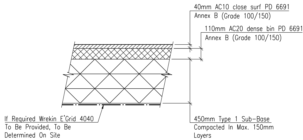
Private Tarmac Construction Detail Scale 1:20
