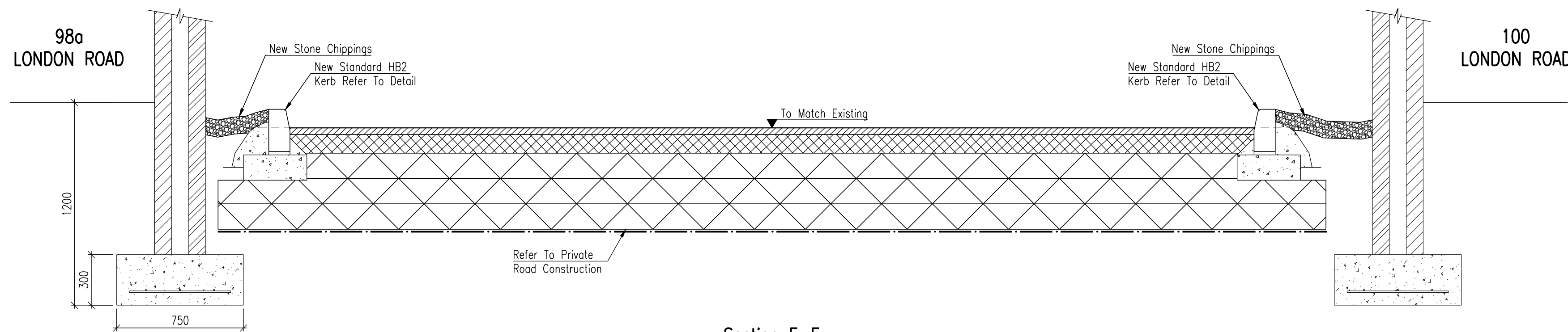
Section E-E Scale 1:20
