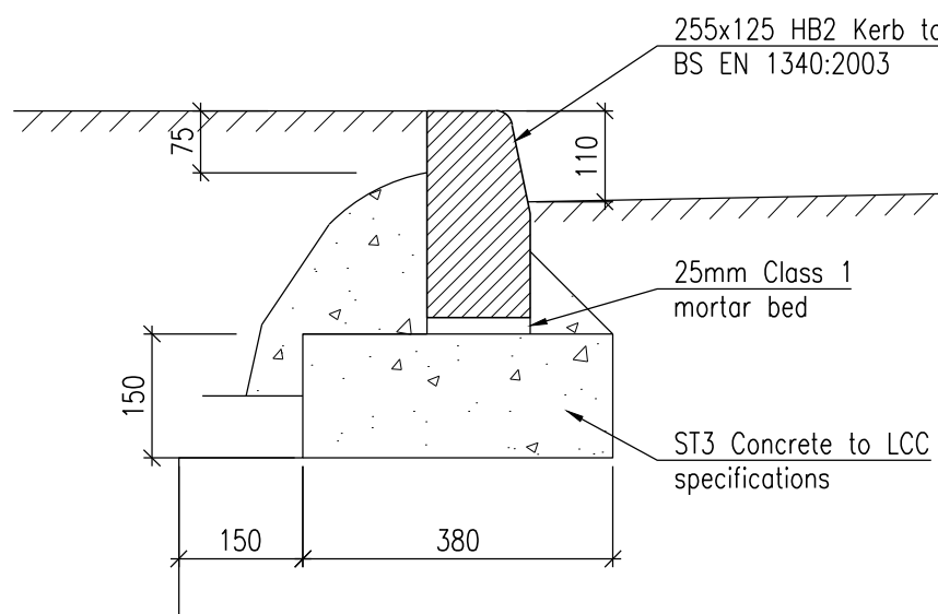
Typical Standard Kerb Detail (125x225 HB) Scale 1:10
