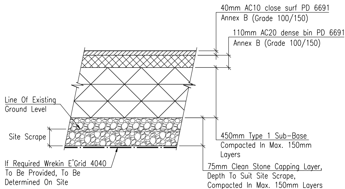
Private Tarmac Construction Detail Where Capping Layer Required Scale 1:20
