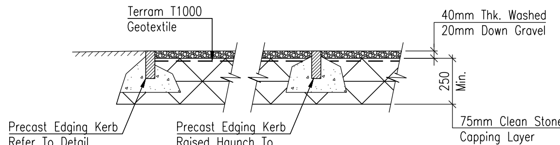
Gravel Surface Detail Scale 1:20
