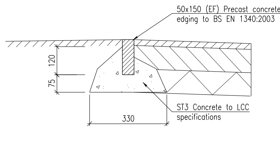
Typical Edging Kerb Detail (50x150 EF) Scale 1:10
