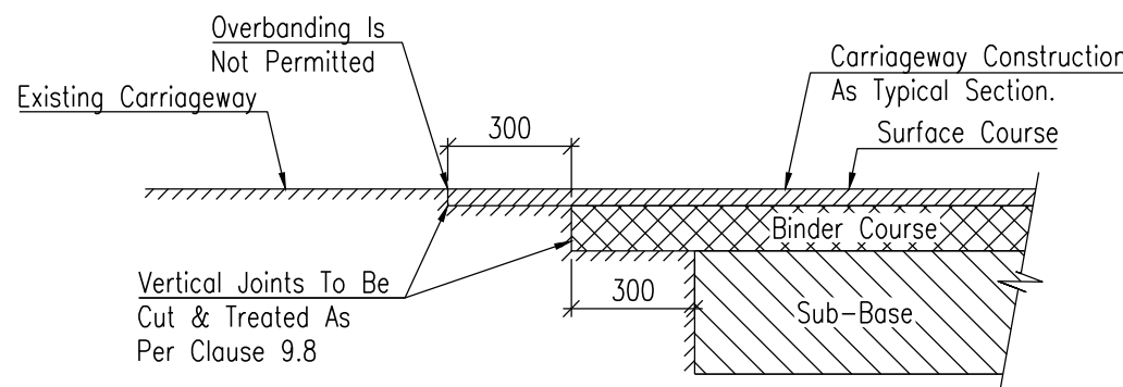
Typical Joint With Existing Carriageways Scale 1:20
