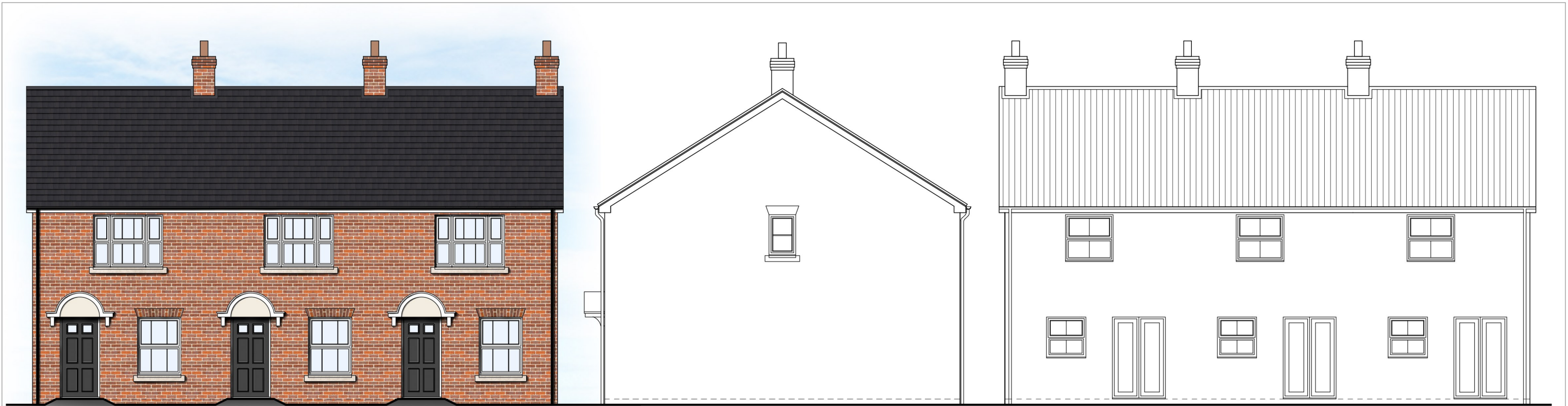
Front Elevation
