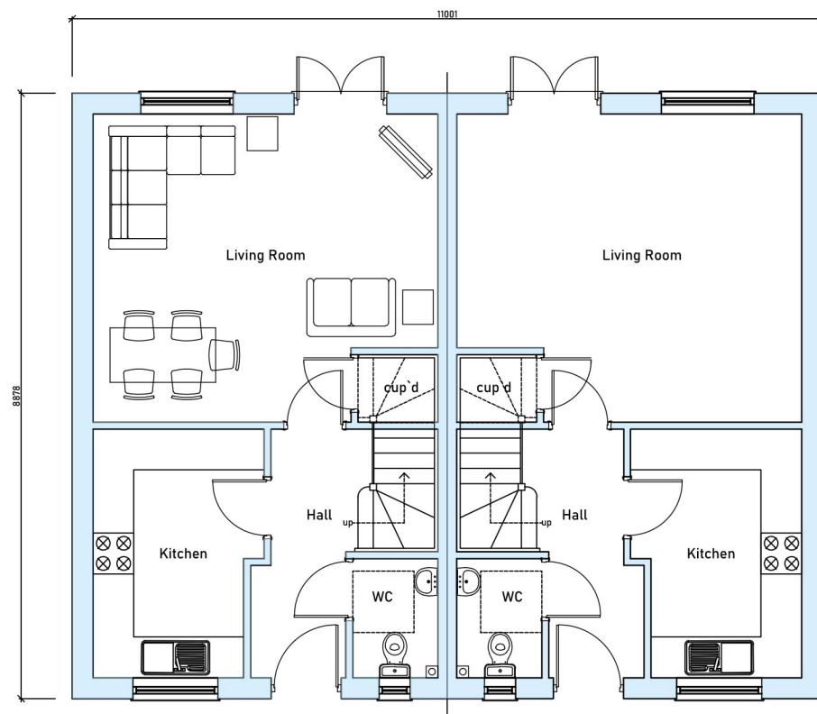
Ground floor plan (83.71m 2 / 901.08ft 2 )
