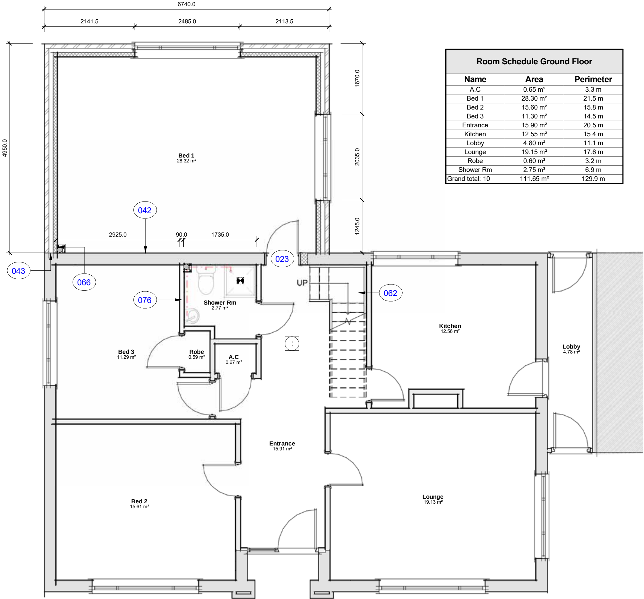
01 - Ground Floor Plan N.T.S
