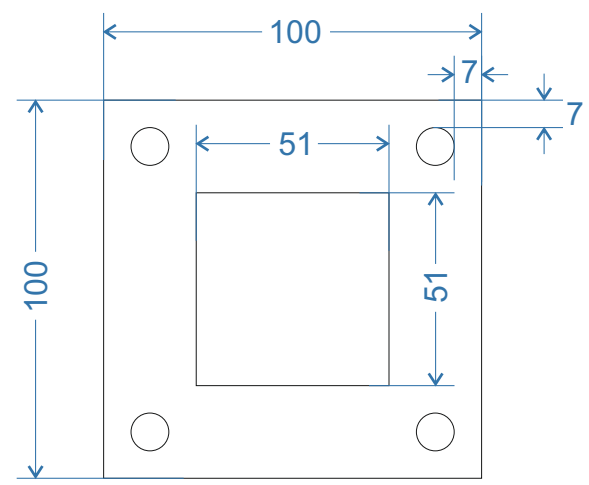
Scale 1:2 5mm steel plate c/w 10mm Ø fixing holes
