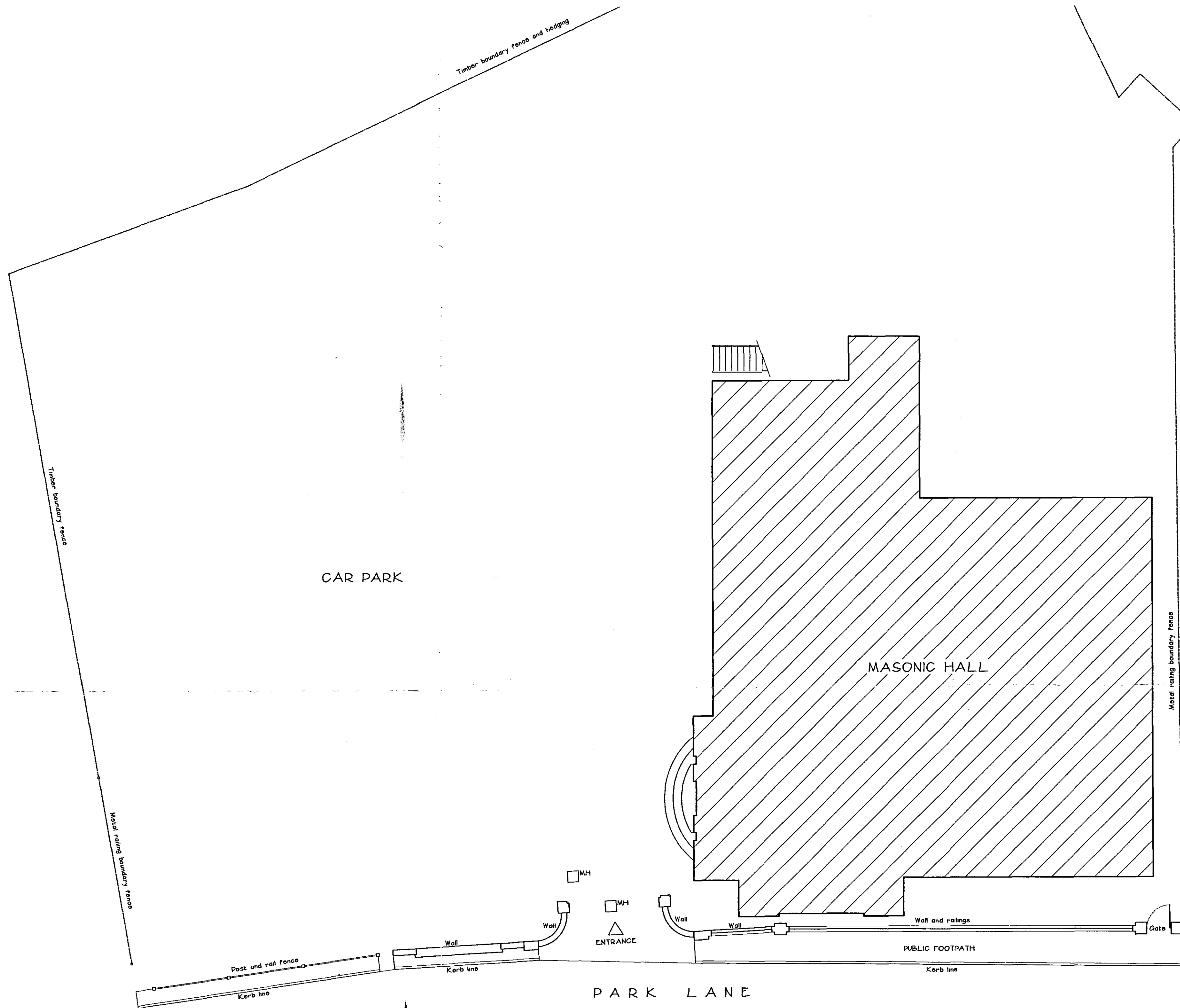
EXISTING BOUNDARY WALL PLAN 1:100
