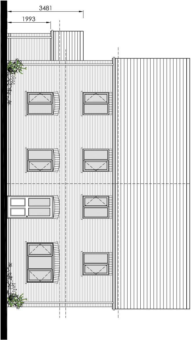
Front Elevation
