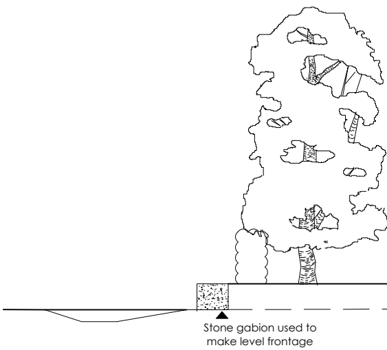
SITE SECTION
