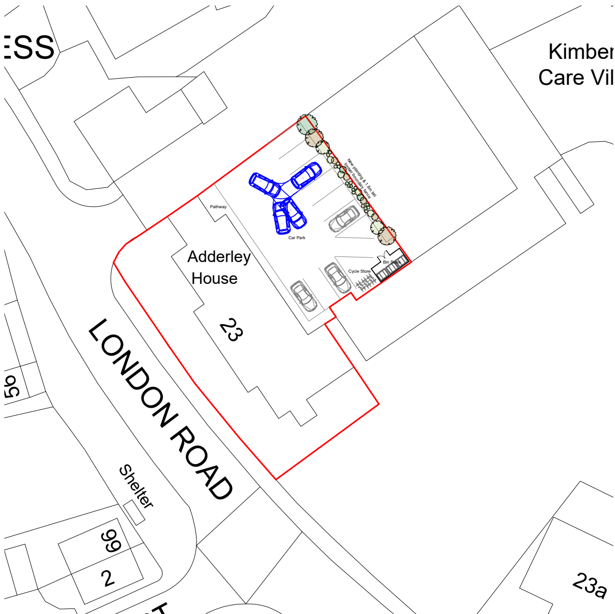
SITE PLAN @ 1:500
