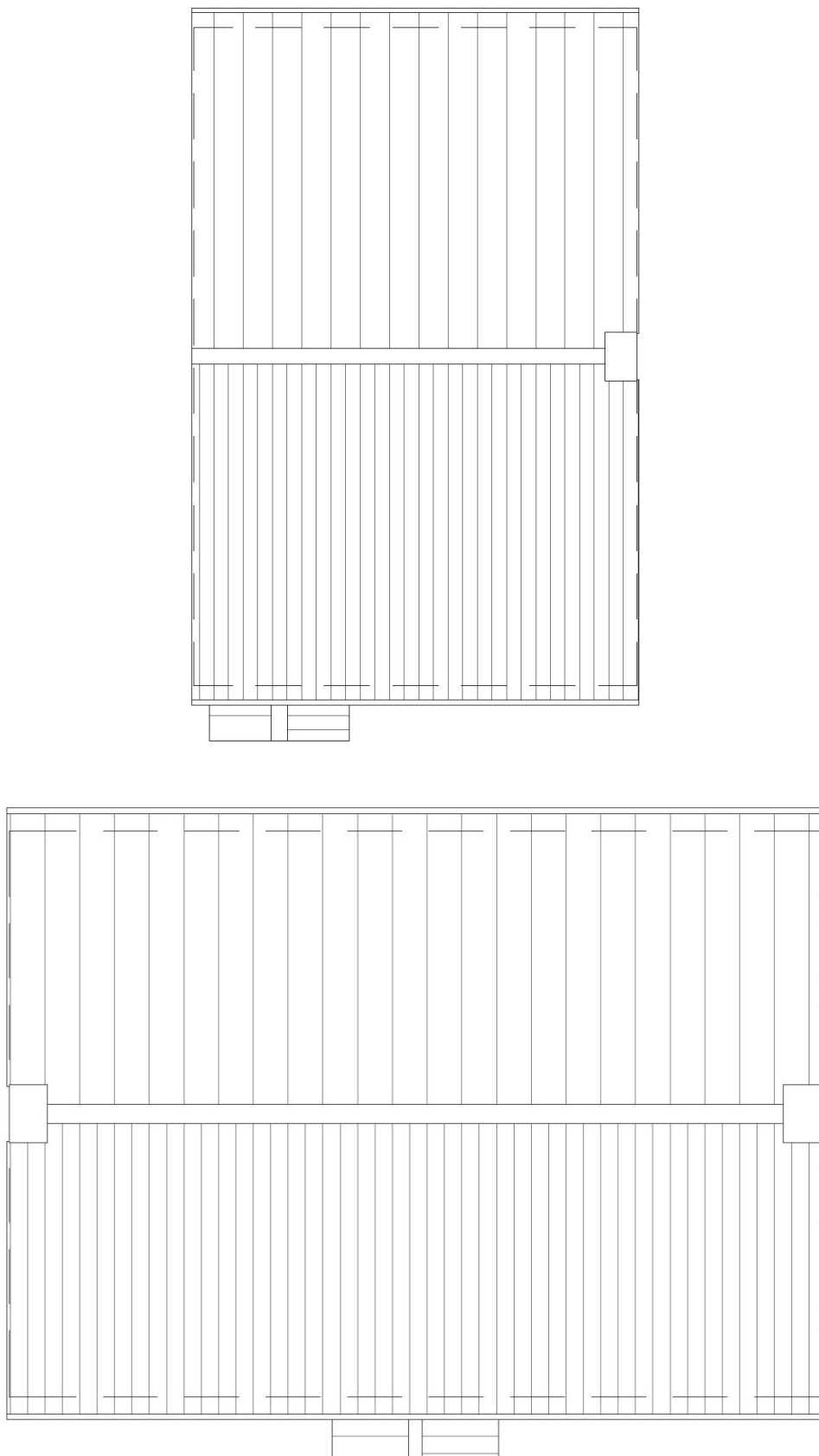
Figure 4: Proposed Roof Plans for 3 bed houses
