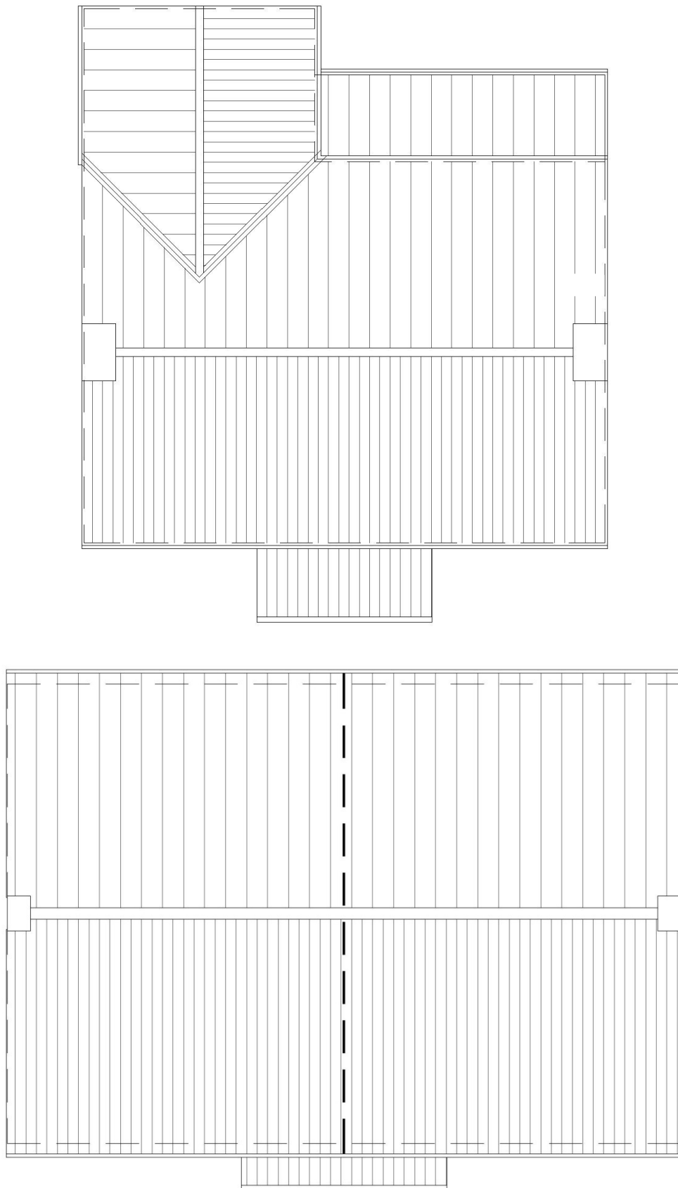
Figure 3 : Proposed Roof Plans for 4 bed & semi-detached houses
