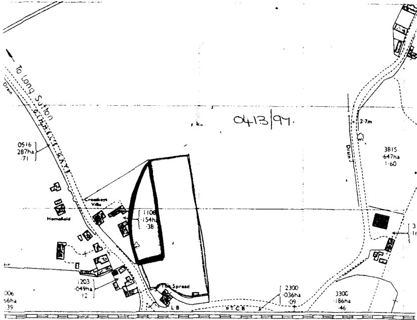
Location Plan 1:2500
