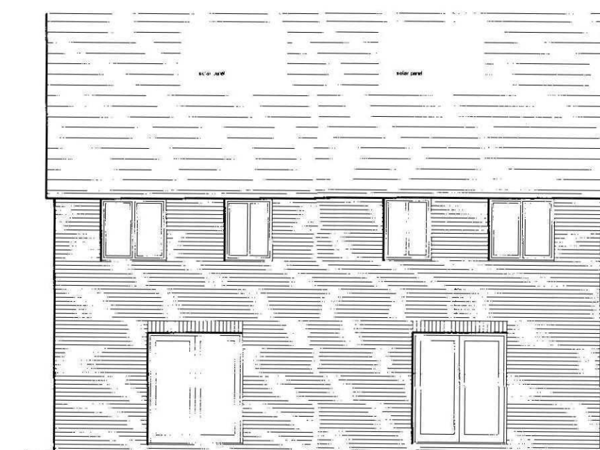
Rear Elevation
