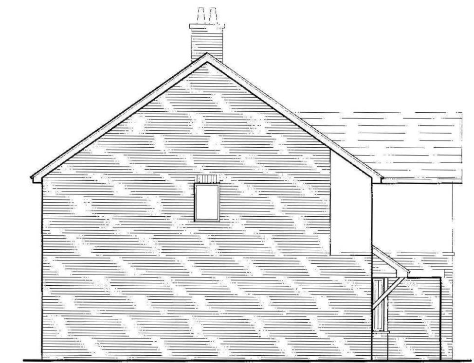
Side Elevation
