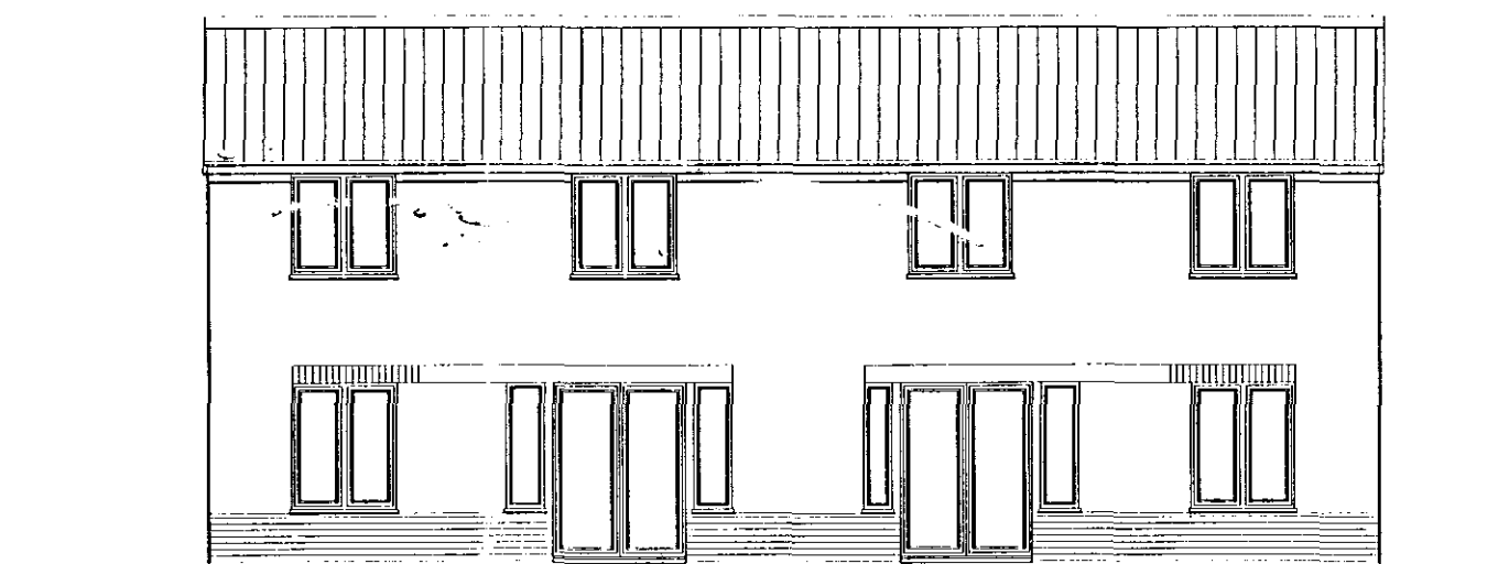
rear elevation
