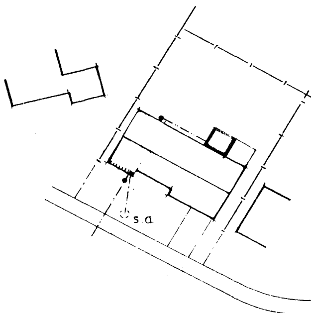
BLOCK PLAN 1:500
