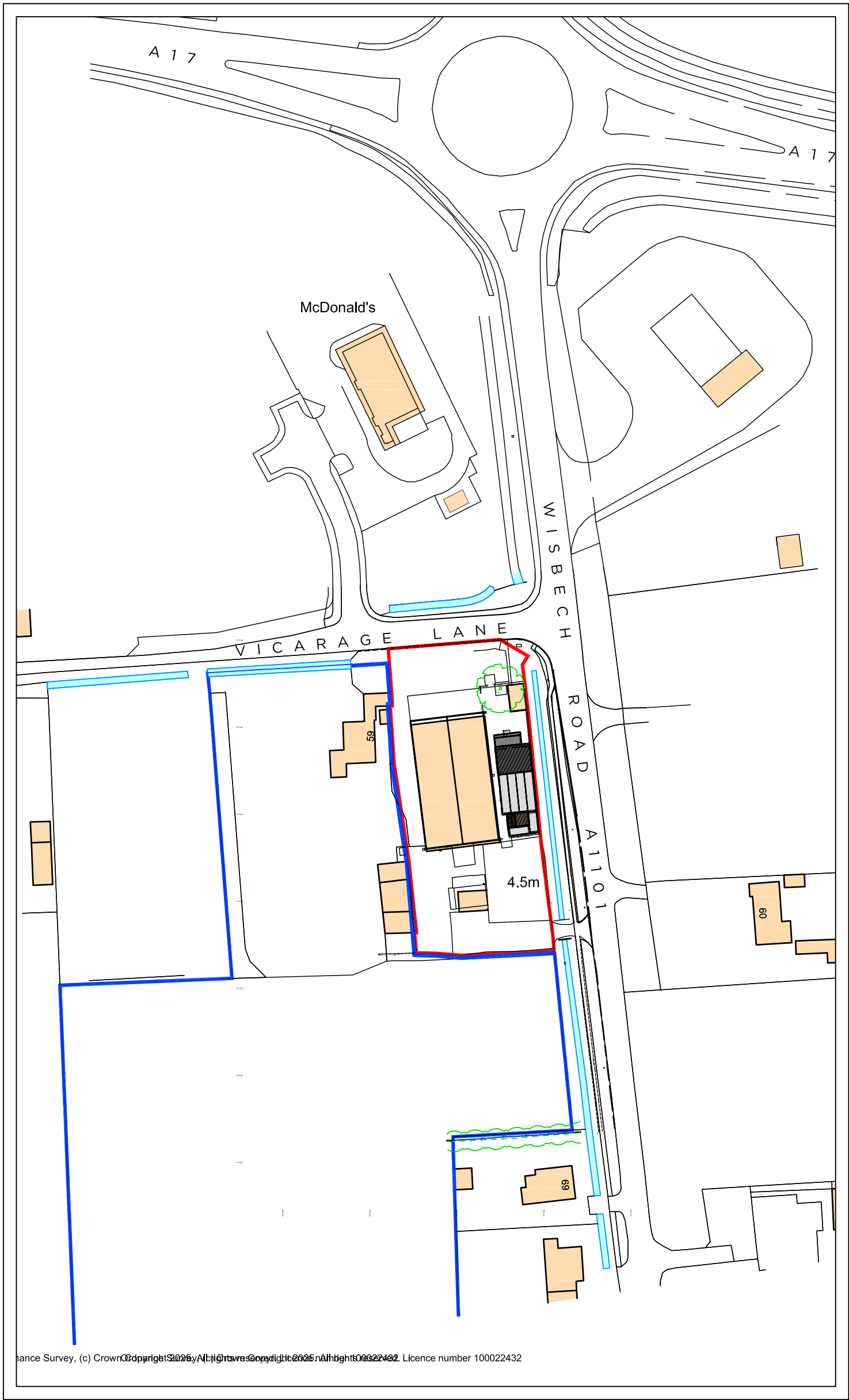
Site Location Plan Scale 1:1250
