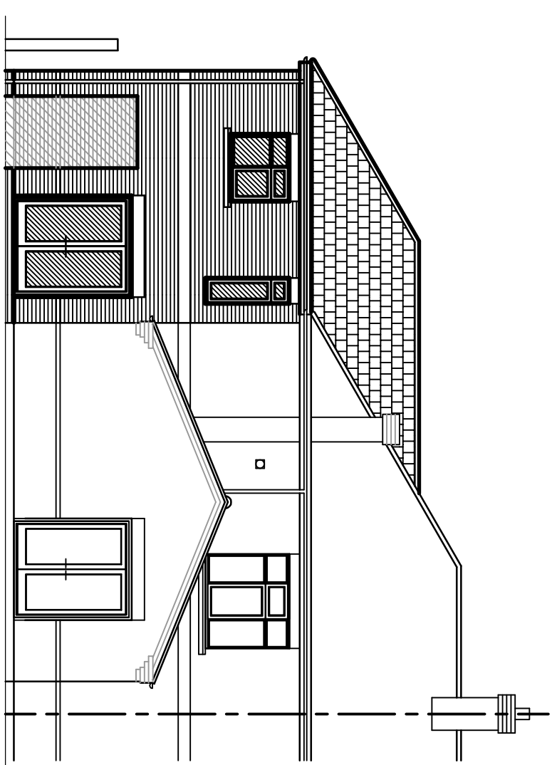
REAR ELEVATION.
