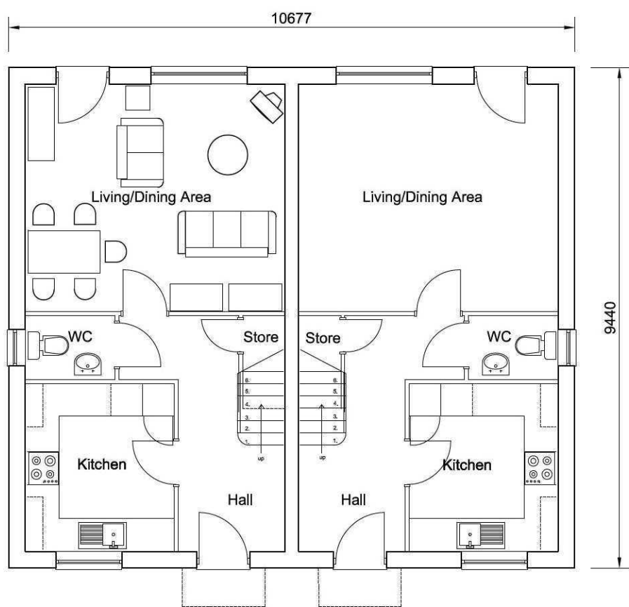
Ground Floor Plan Plots 32 & 33
