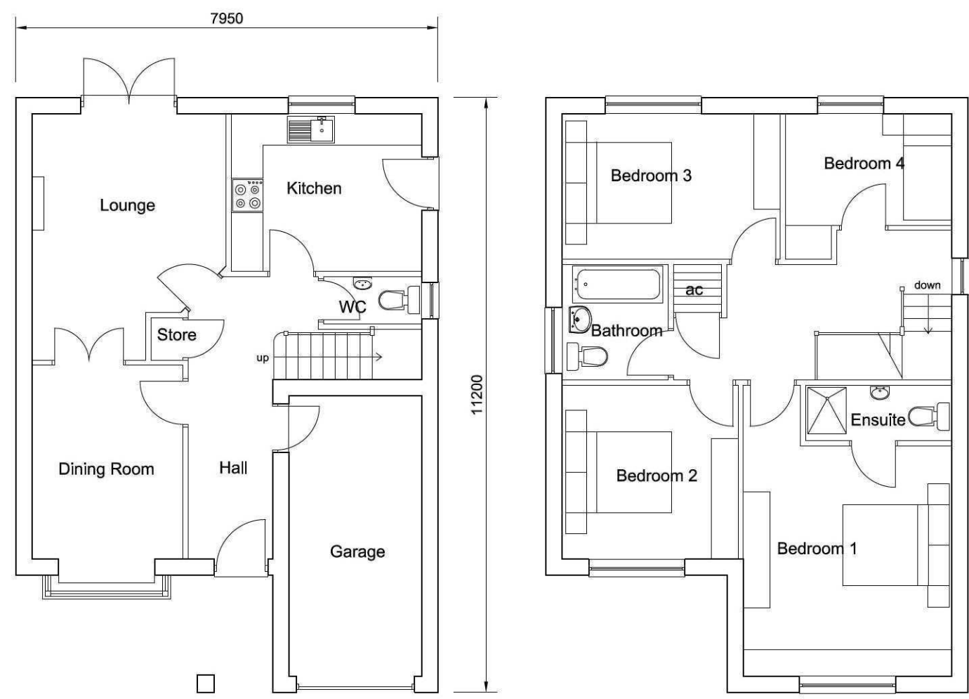
Ground Floor Plan Plot 3, 50 & 74 plot 75 mirrored
