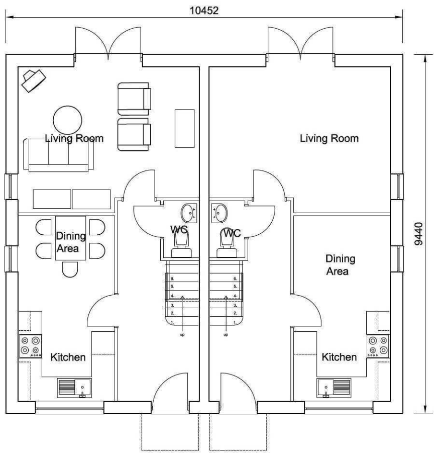
Ground Floor Plan Plots 4 & 5, & 6 & 7
