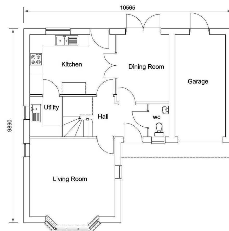
Ground Floor Plan Plots 2, & 73 plots 66, 71, & 72 mirrored
