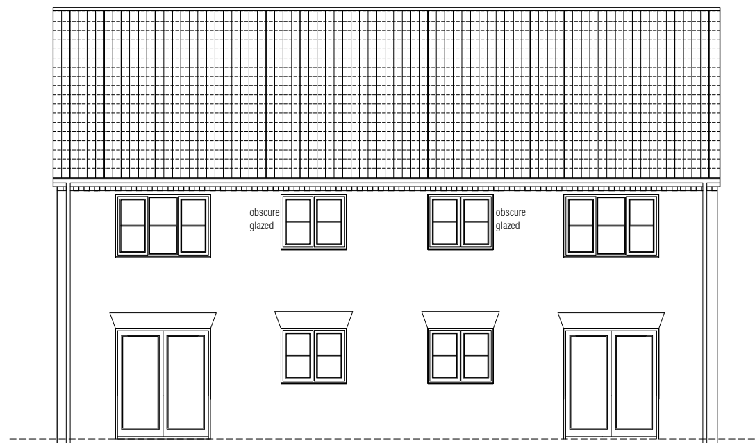
rear elevation
