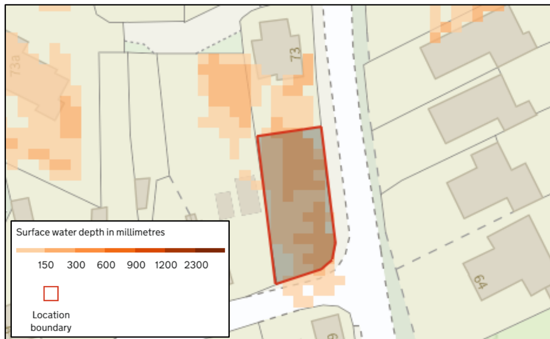
Figure 3 – 2061-2125 1 in 100 Annual Likelihood of Surface Water Flooding
