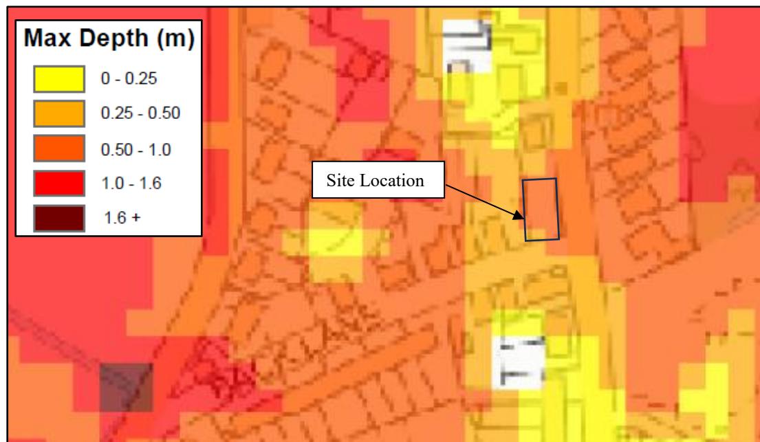
Figure 4 – SFRA 2116 Residual Peak Depth Map (0.1% annual probability)
