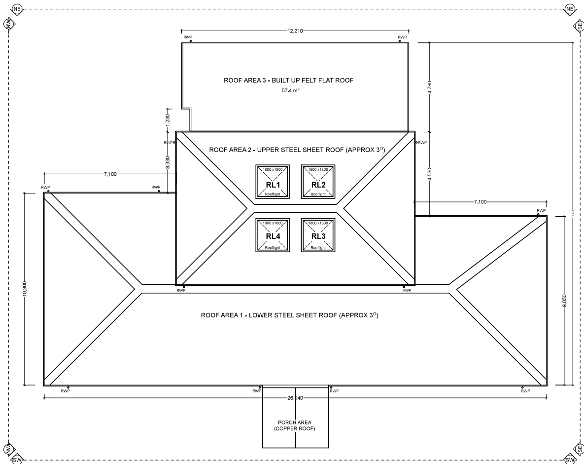
ROOF PLAN AS EXISTING @ 1:100
