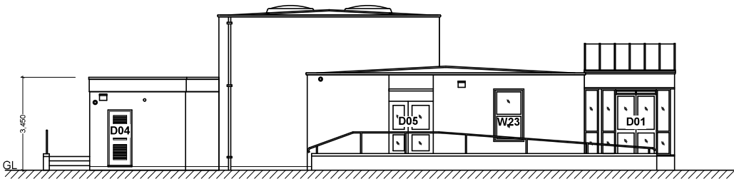
NORTH WEST ELEVATION AS EXISTING @ 1:100
