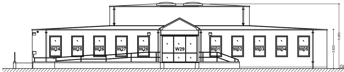
SOUTH WEST ELEVATION AS EXISTING @ 1:100
