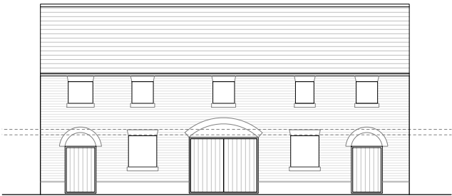
FRONT ELEVATION @ 1:200
