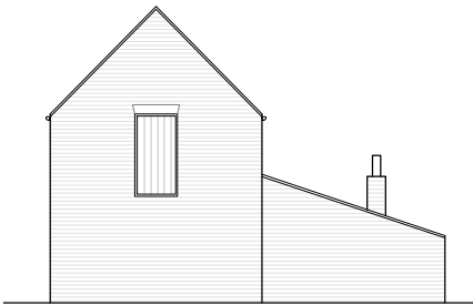
RIGHT ELEVATION @ 1:200
