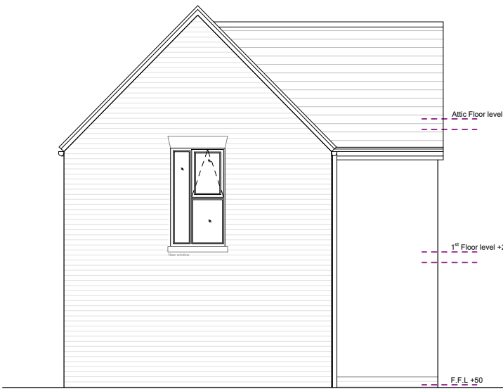
RIGHT GABLE ELEVATION @ 1:100
