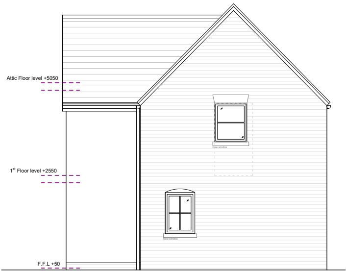
LEFT GABLE ELEVATION @ 1:100
