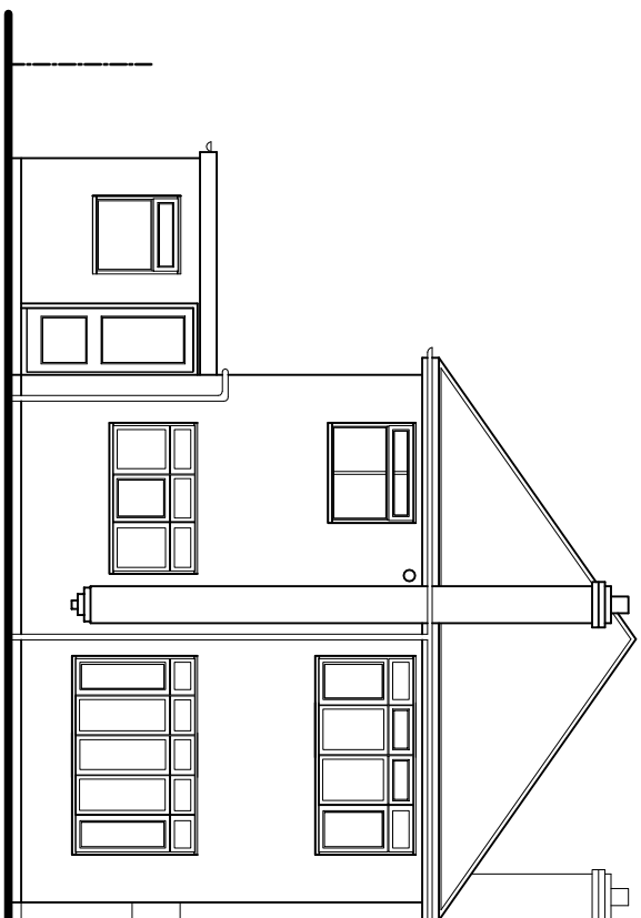
REAR ELEVATION.
