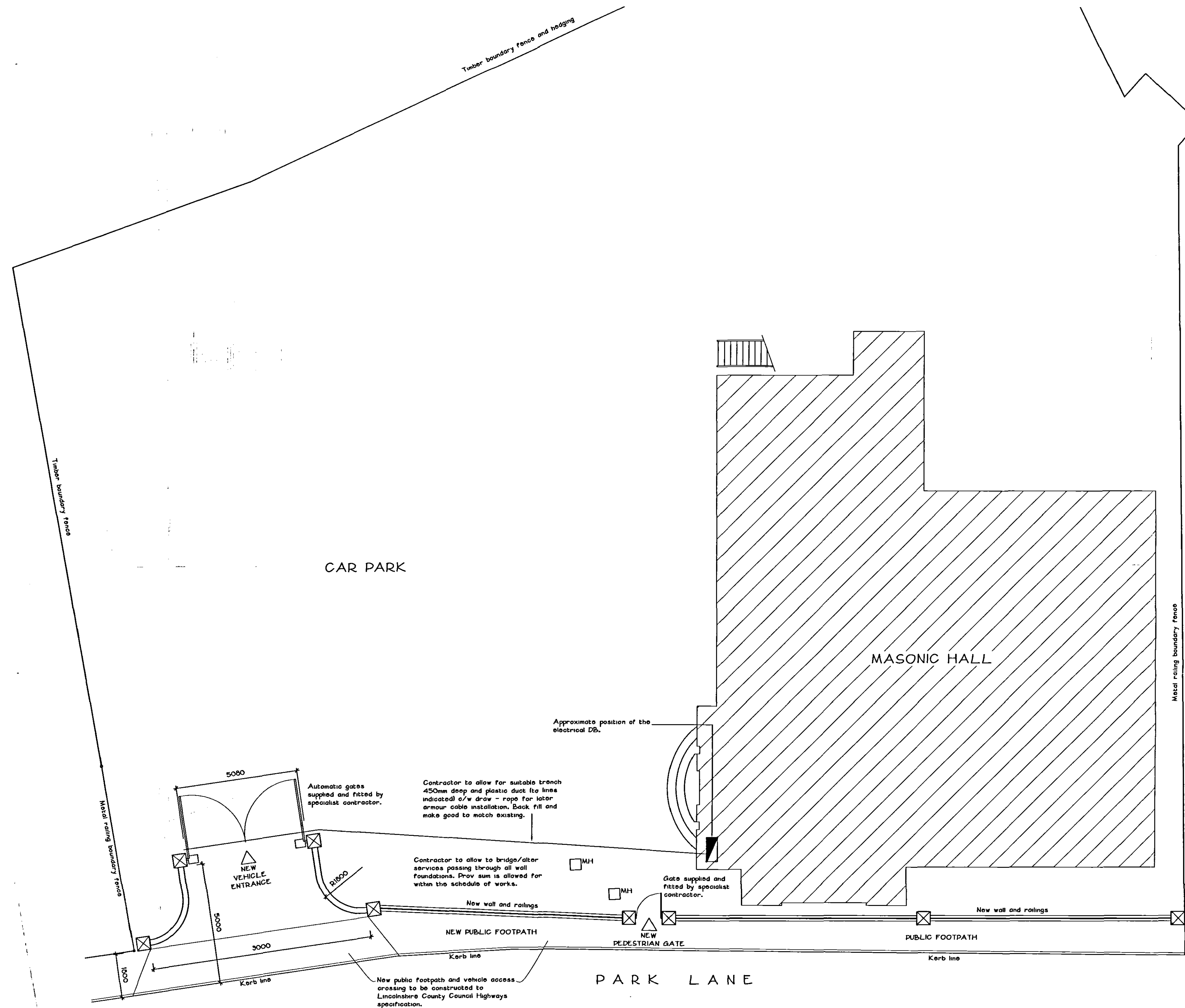
PROPOSED BOUNDARY WALL PLAN 1:100
