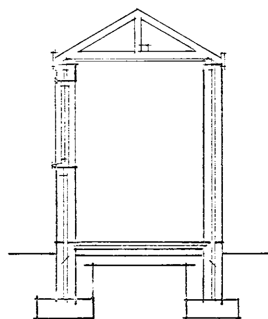
SECTION THRO PORCH
