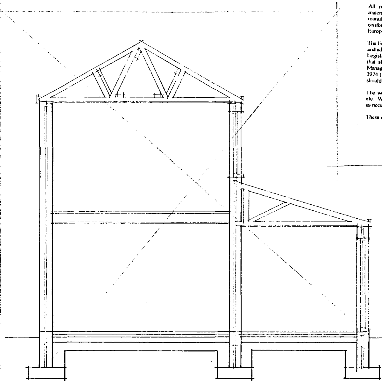
SECTION
