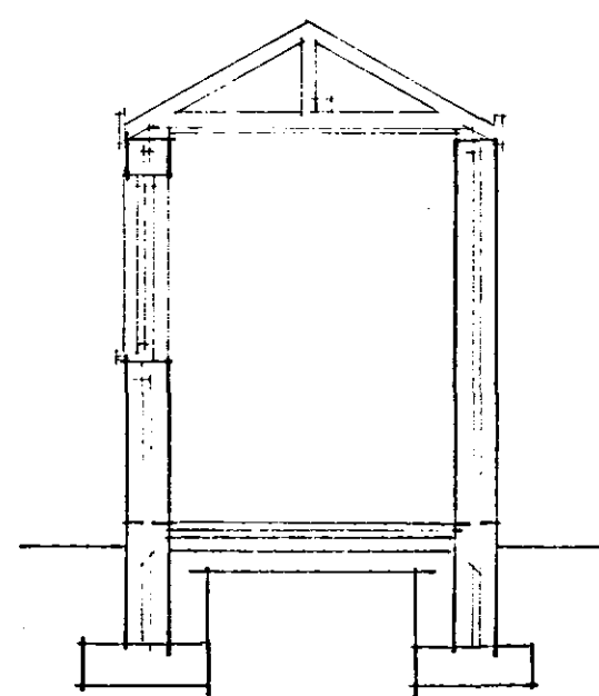
SECTION THRO PORCH
