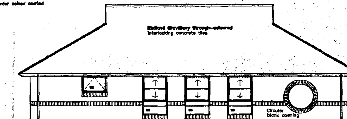
ELEVATION TO CLASSROOM
