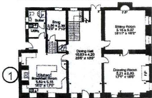
Ground Floor
