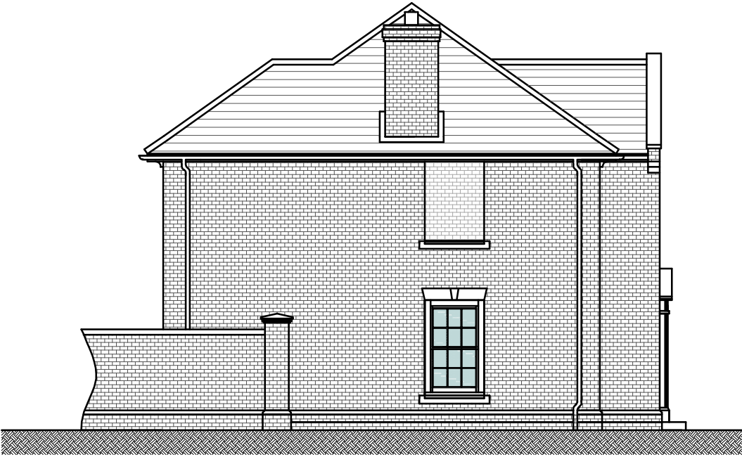
SOUTH ELEVATION
