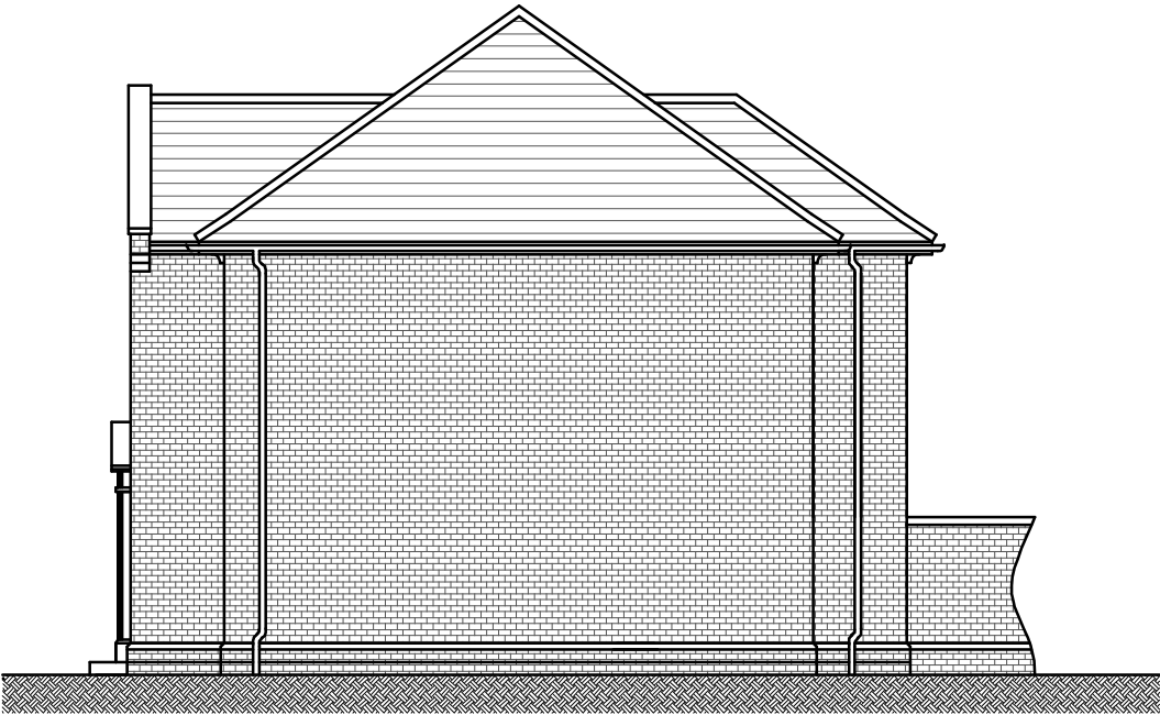
NORTH ELEVATION
