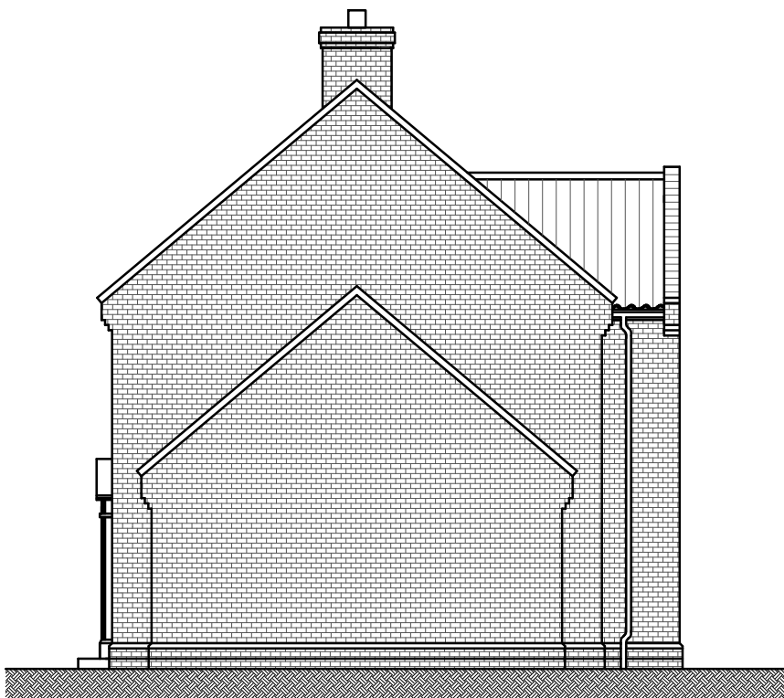
NORTH ELEVATION
