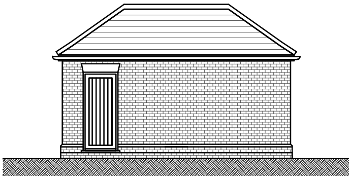
EAST ELEVATION
