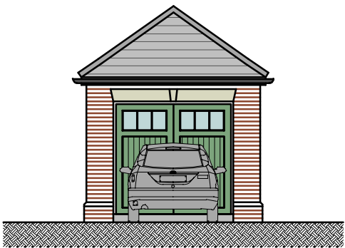
SOUTH ELEVATION
