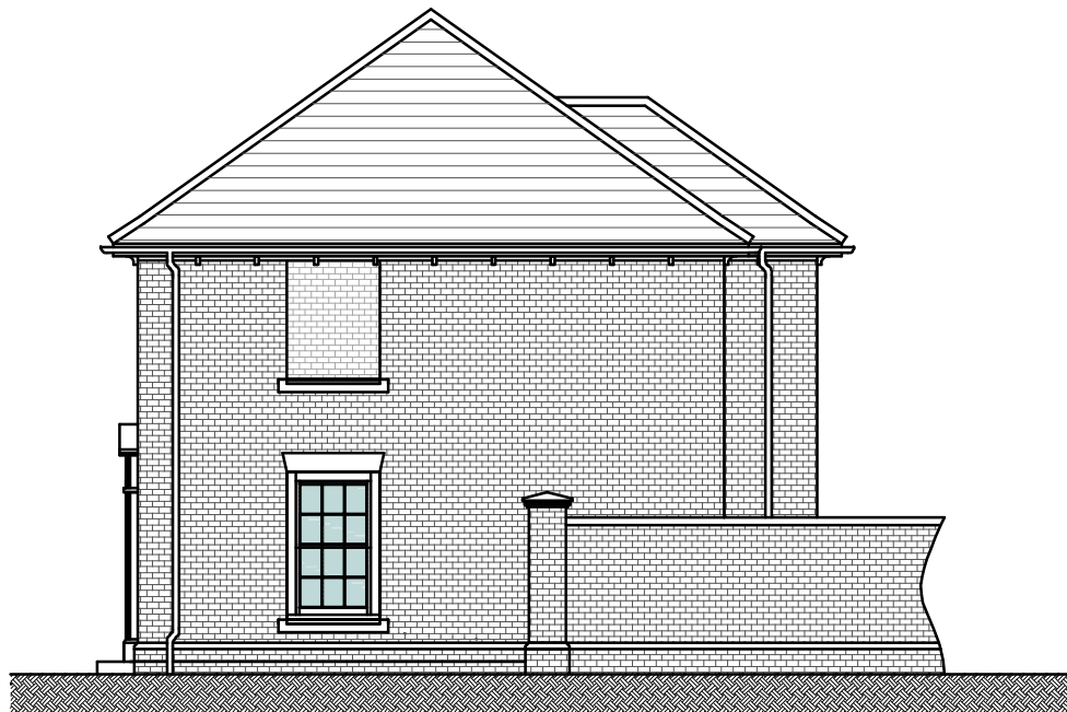
NORTH ELEVATION
