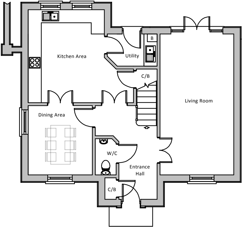
GROUND FLOOR LAYOUT PLAN
