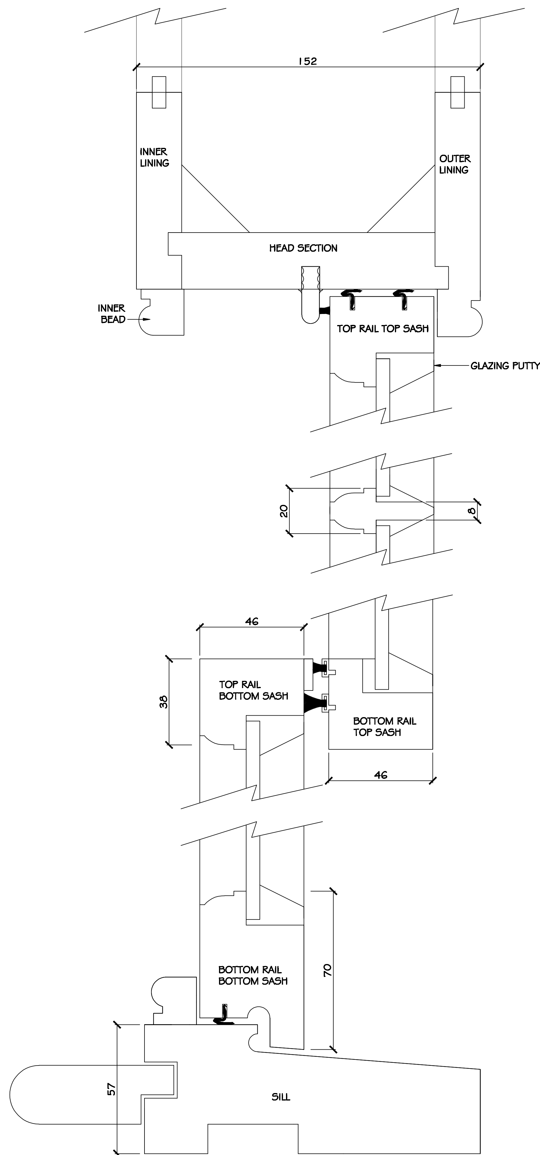
VERTICAL SECTION
