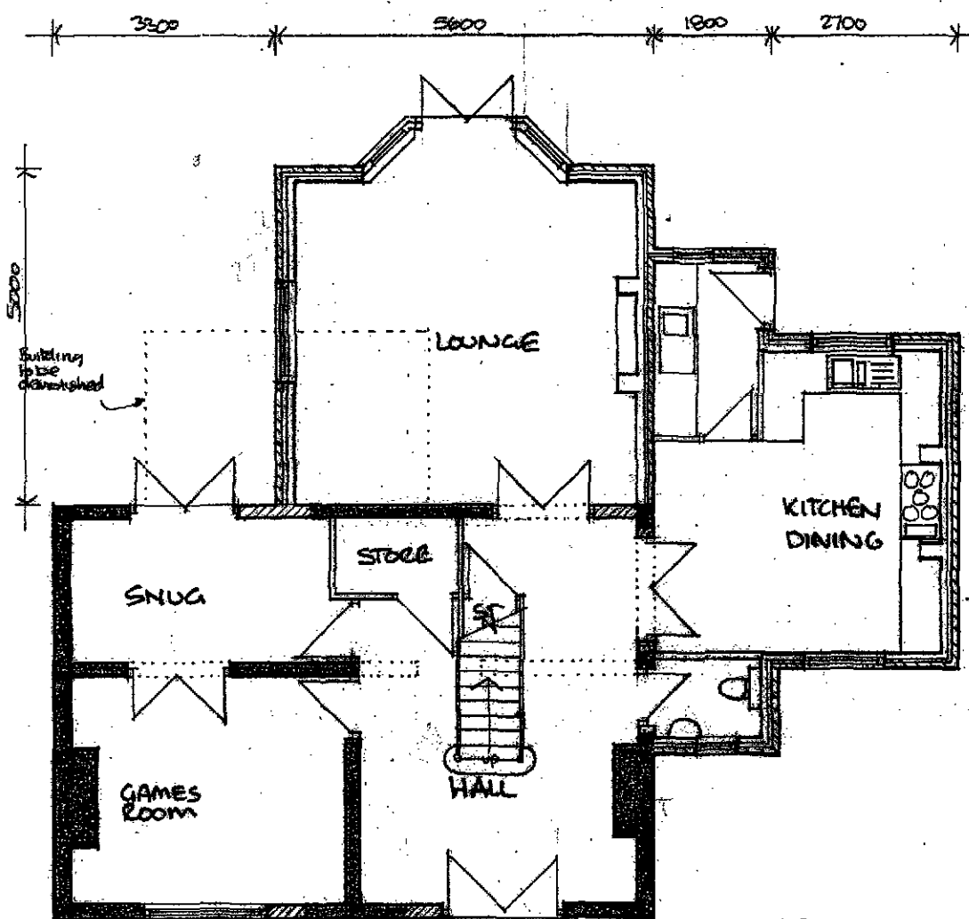
GROUND FLOOR
