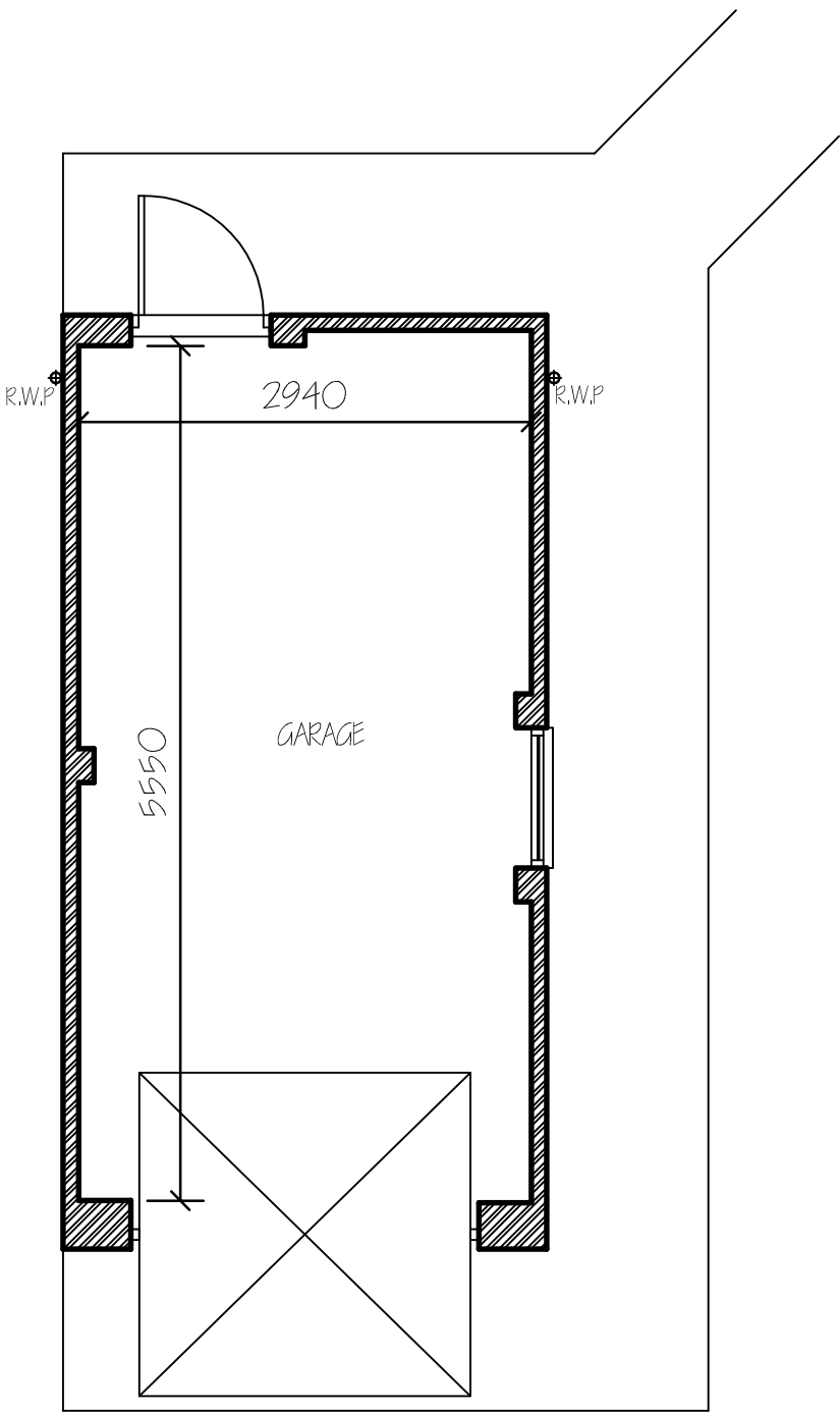
FLOOR PLAN
