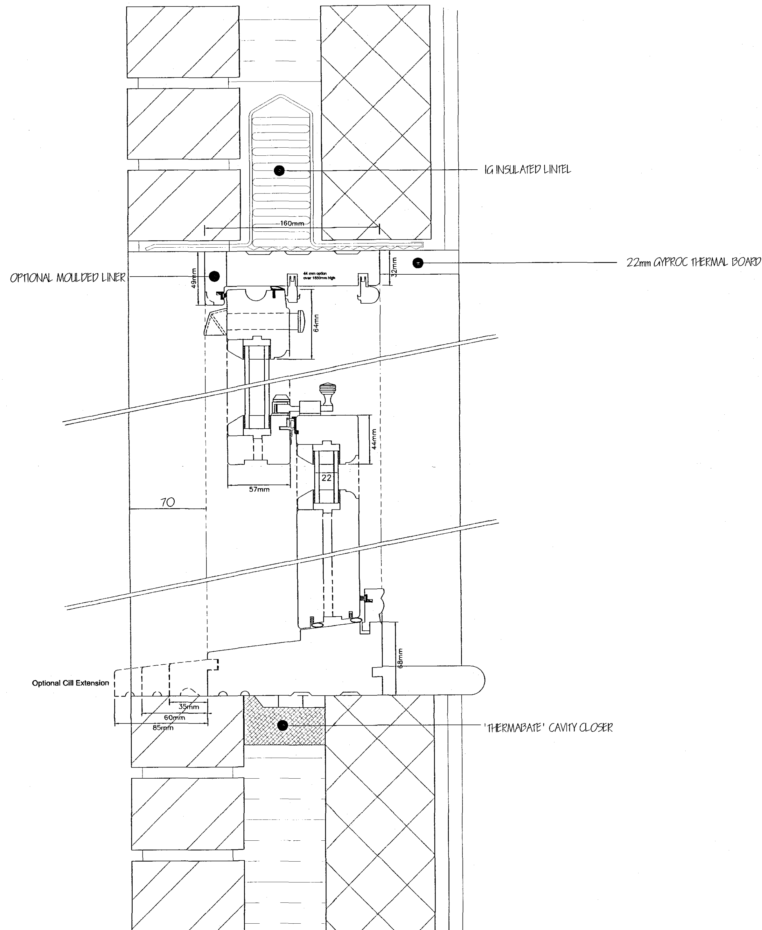
TYPICAL SECTION THROUGH WINDOW 1:2
