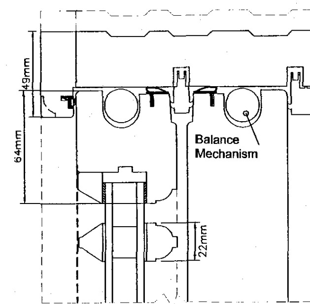
TYPICAL SECTION THROUGH JAMB 1:2
