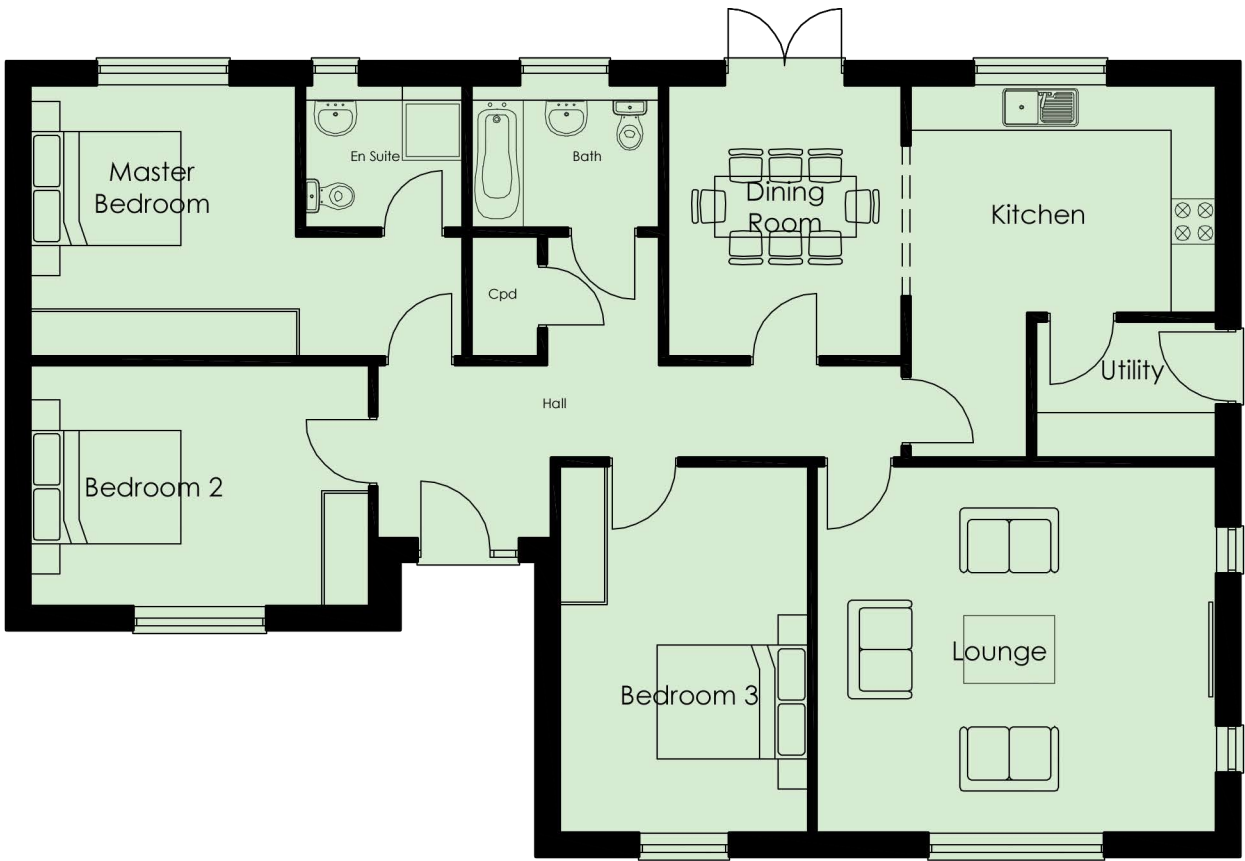
Floor Plan
