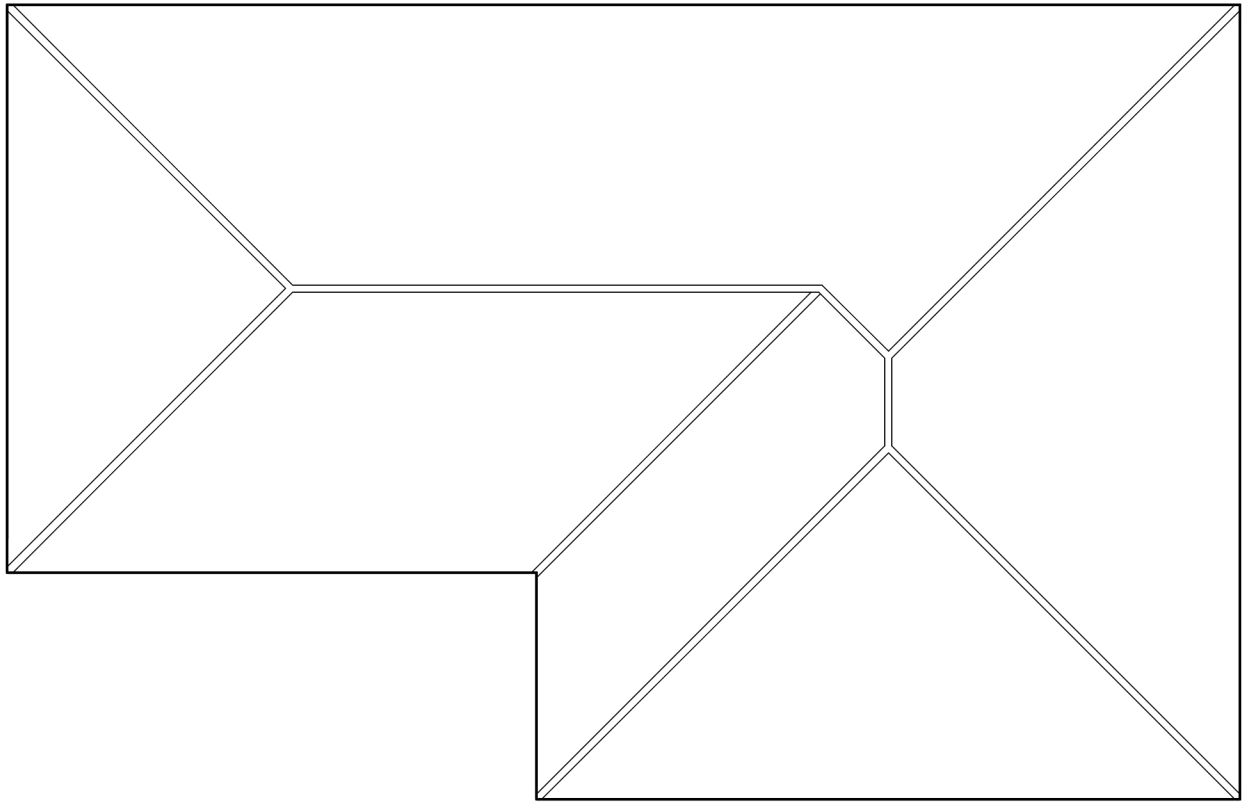
Roof Plan
