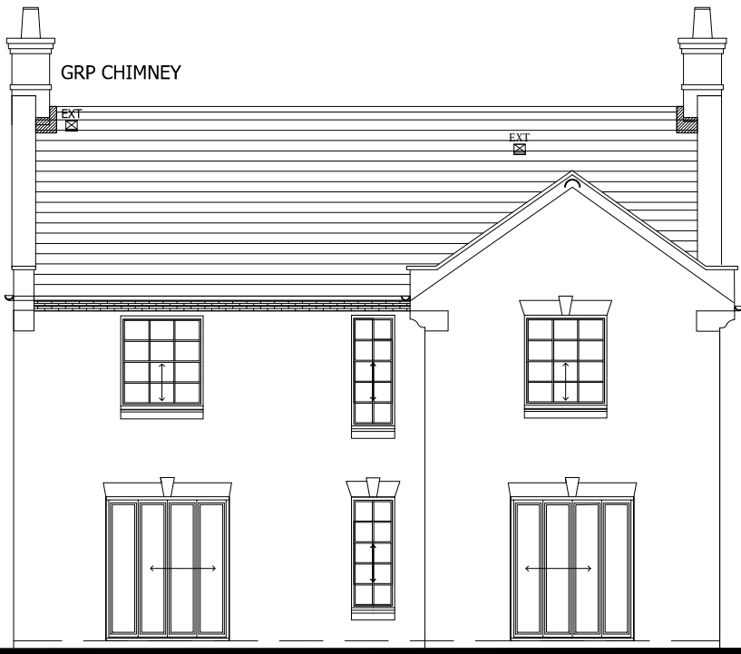
REAR ELEVATION
