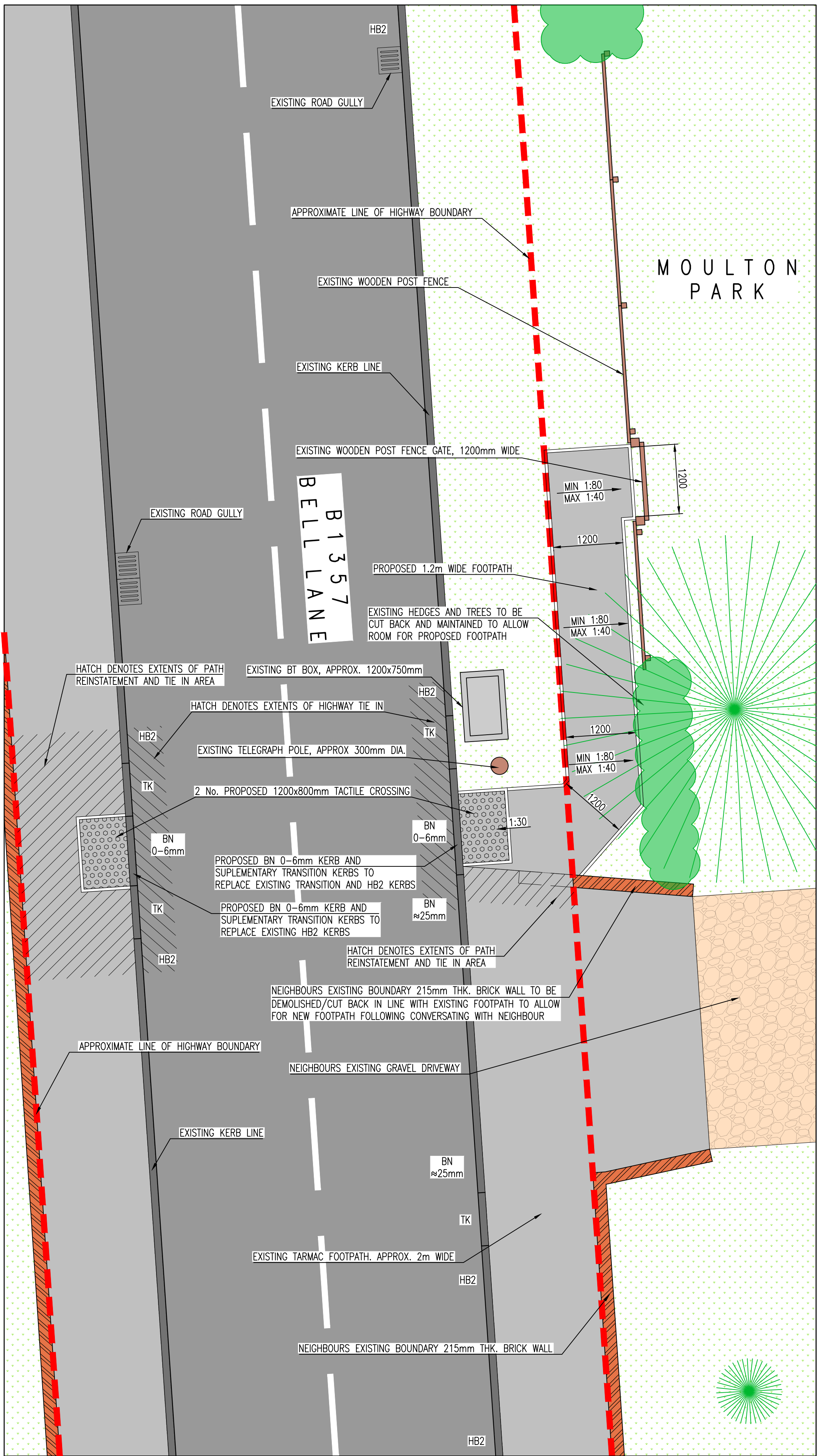
PROPOSED FOOTPATH LAYOUT SCALE 1:50
