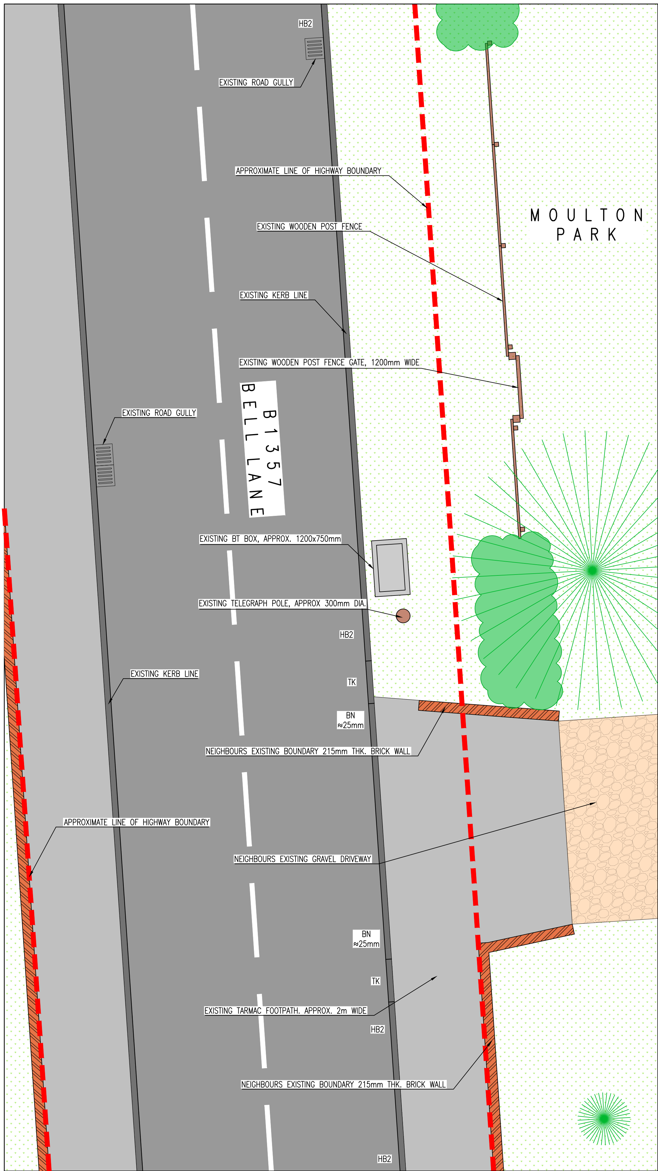
EXISTING FOOTPATH LAYOUT SCALE 1:50
