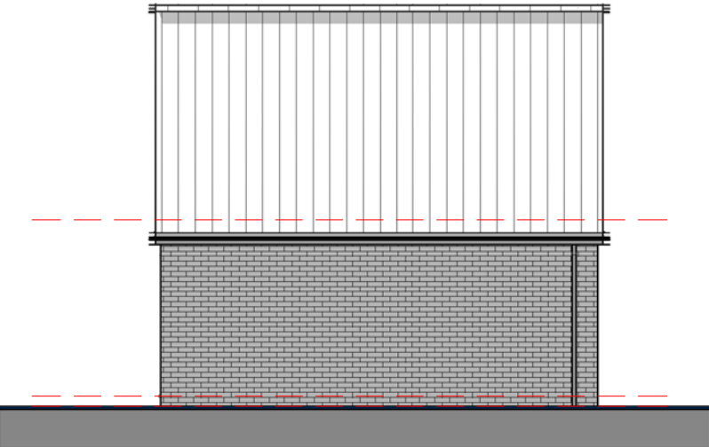
Elevation 03 - Rear 1 : 100
