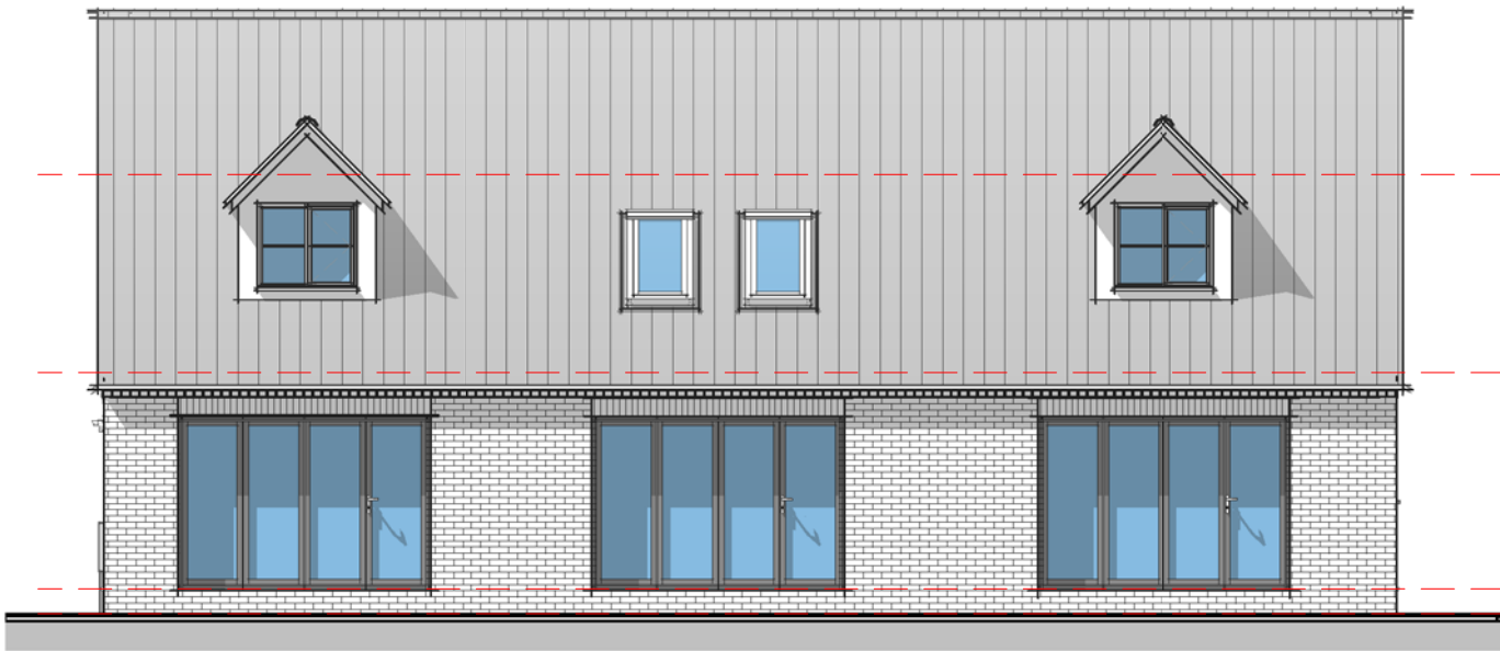
Elevation 03 - Rear
