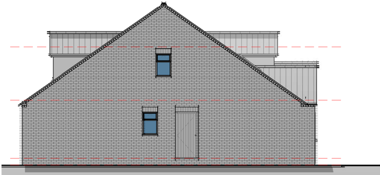
Elevation 04 - Left
