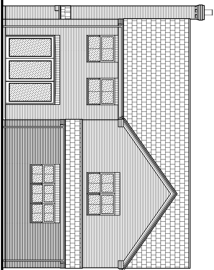
REAR ELEVATION
