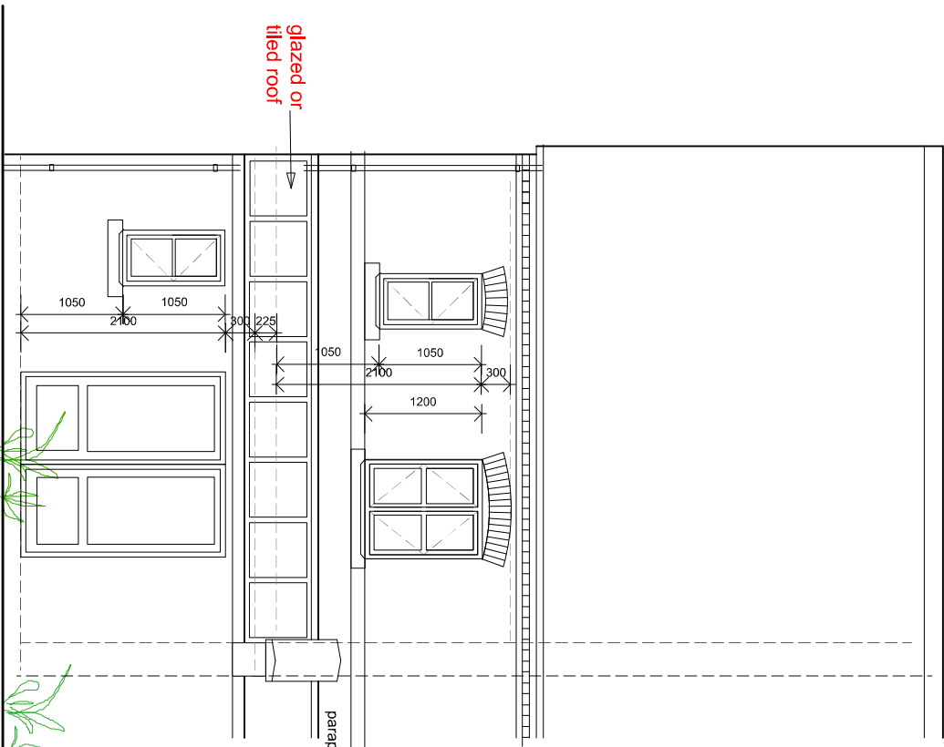
REAR ELEVATION
