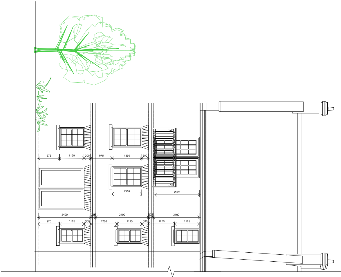
REAR ELEVATION
