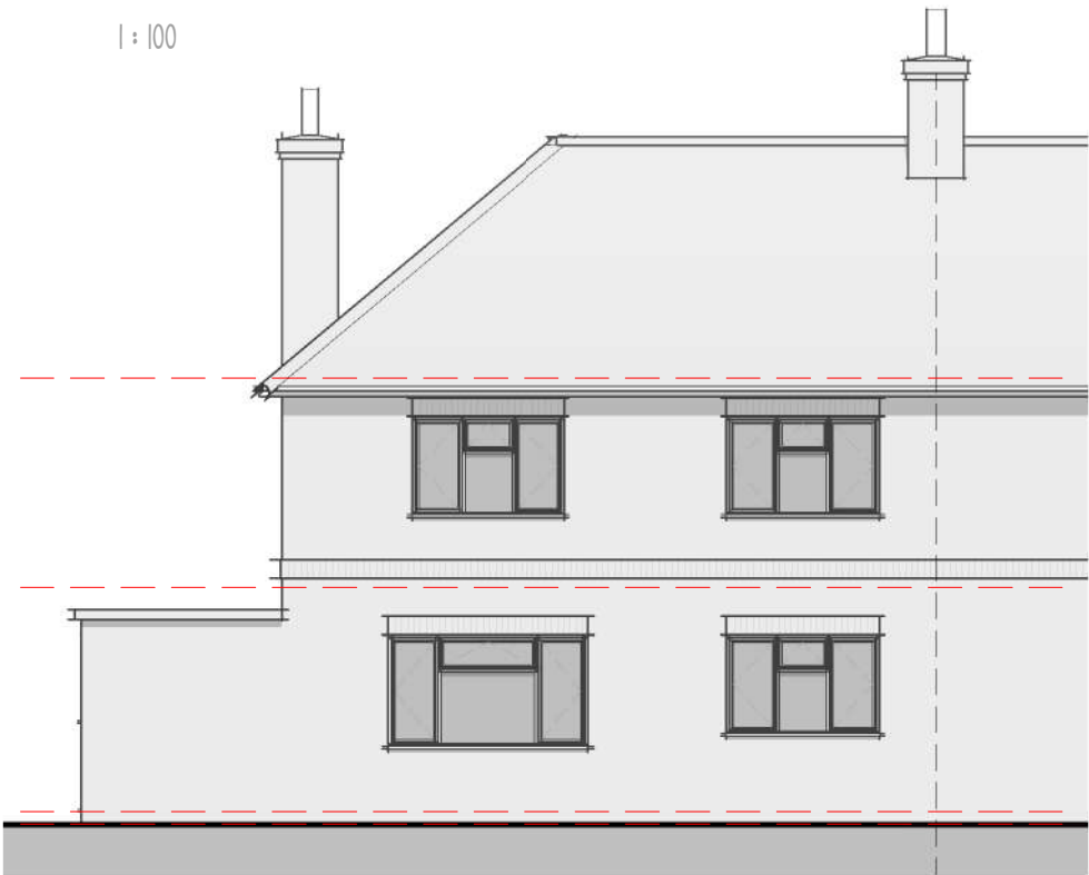
Elevation 03 - Rear
