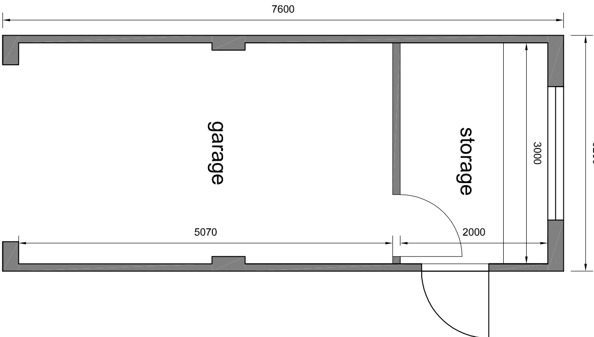
PROPOSED GARAGE FLOOR PLAN
