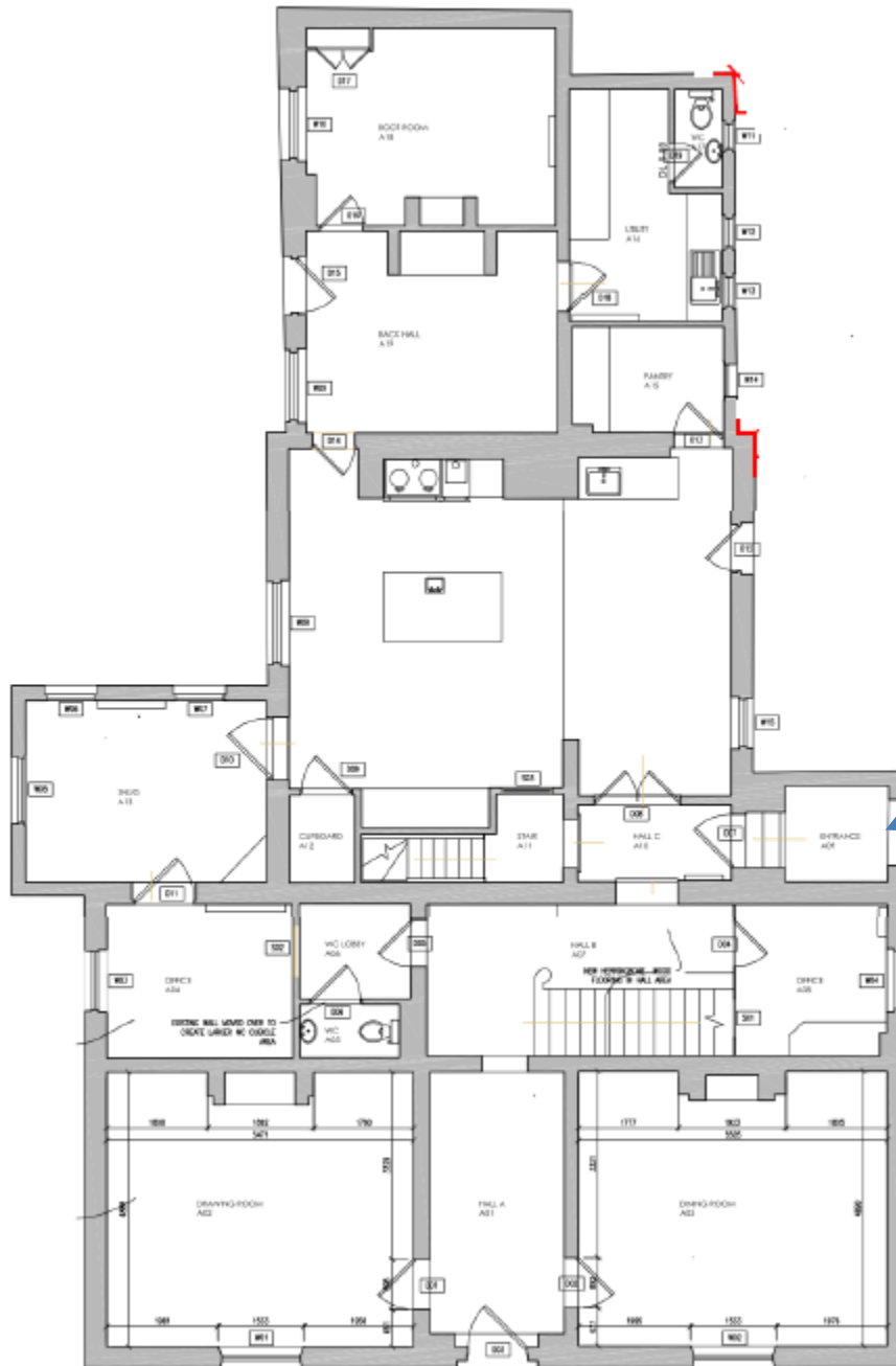
Ground Floor
