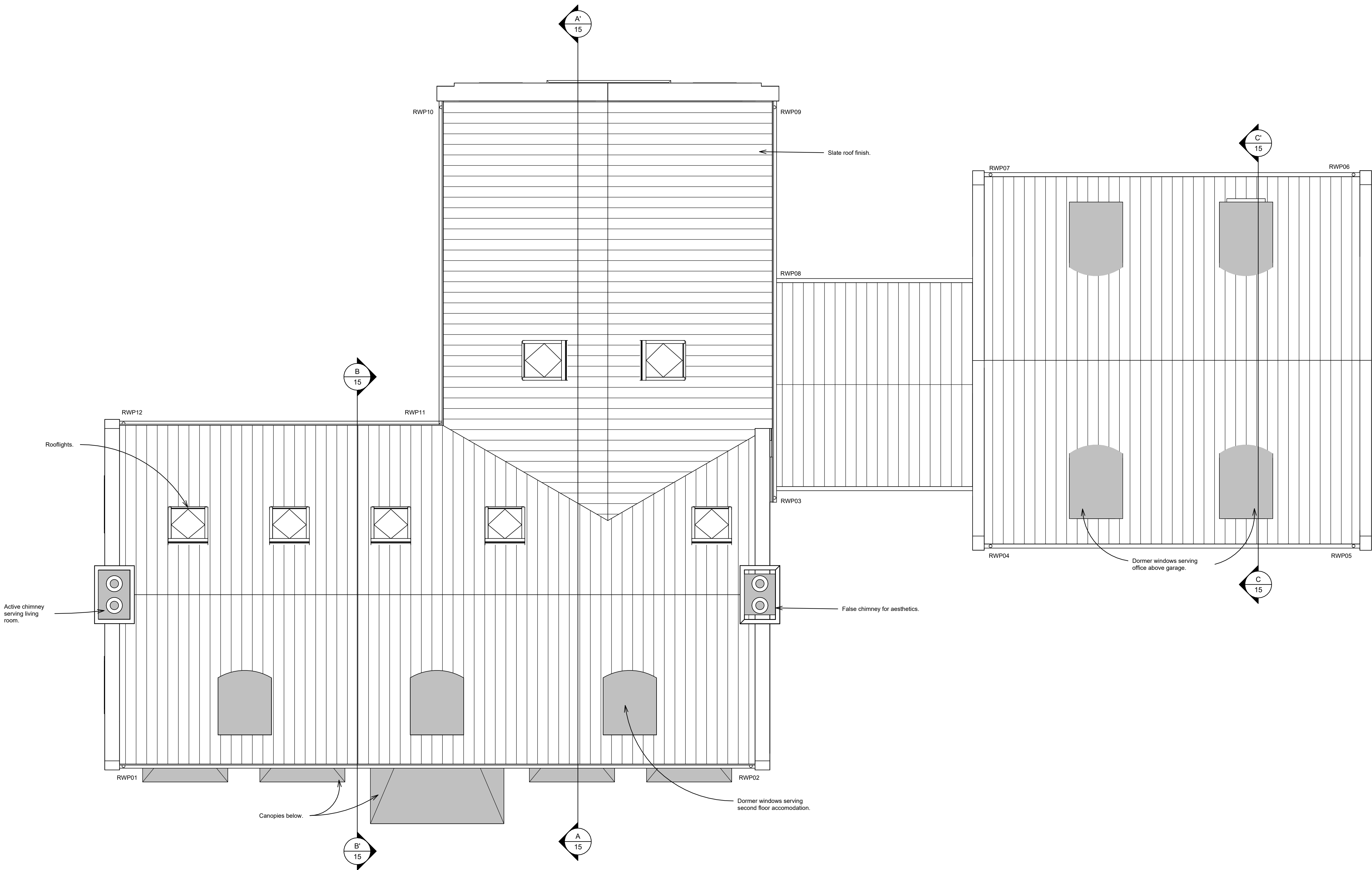
Roof Finishes Plan as proposed Scale 1 : 50
